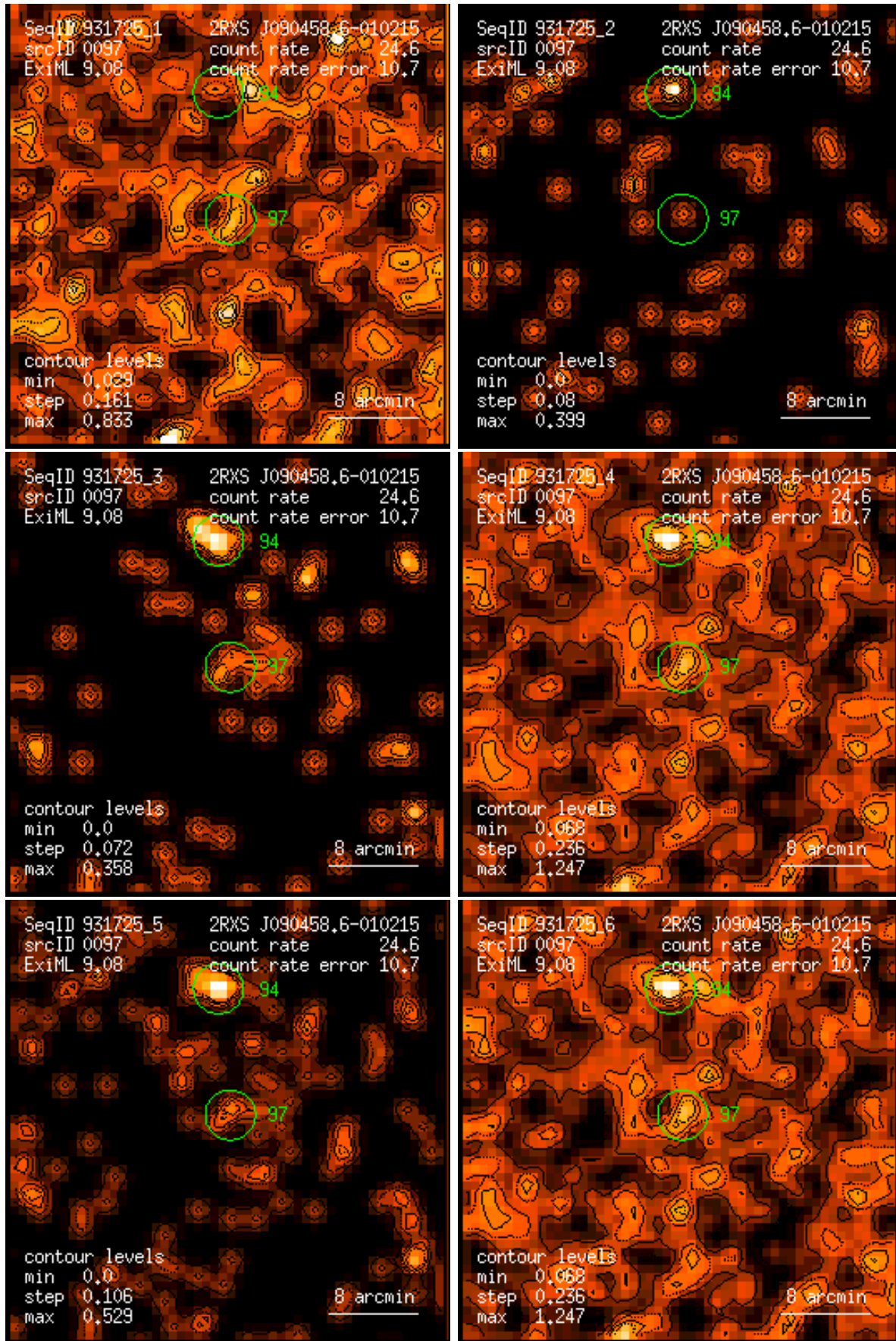
Figure 97: RASS 931725: detection 0097: band rate images, Gaussian filter: (1) PSPC channels 11 – 41, (2) 52 – 90, (3) 91 – 201, (4) 11 – 235, (5) 52 – 201, (6) 11 – 201. Broad band rates in counts/ks. Band rate contour levels in counts/ks/arcmin 2 .
