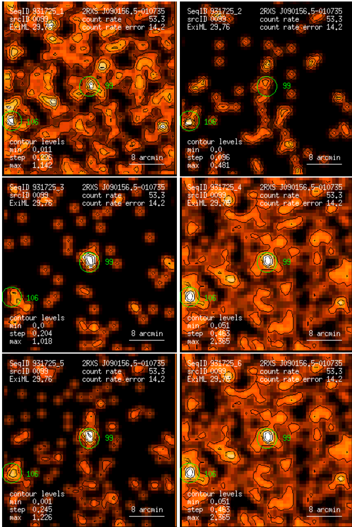
Figure 99: RASS 931725: detection 0099: band rate images, Gaussian filter: (1) PSPC channels 11 – 41, (2) 52 – 90, (3) 91 – 201, (4) 11 – 235, (5) 52 – 201, (6) 11 – 201. Broad band rates in counts/ks. Band rate contour levels in counts/ks/arcmin 2 .
