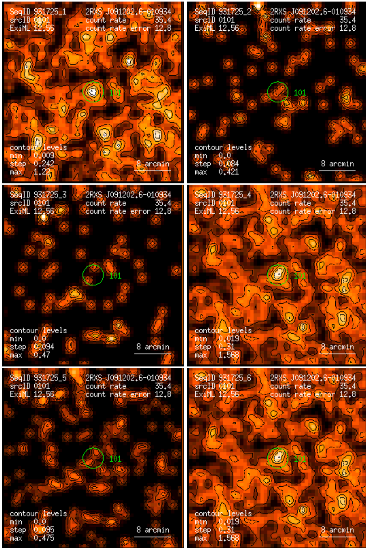
Figure 101: RASS 931725: detection 0101: band rate images, Gaussian filter: (1) PSPC channels 11 – 41, (2) 52 – 90, (3) 91 – 201, (4) 11 – 235, (5) 52 – 201, (6) 11 – 201. Broad band rates in counts/ks. Band rate contour levels in counts/ks/arcmin 2 .
