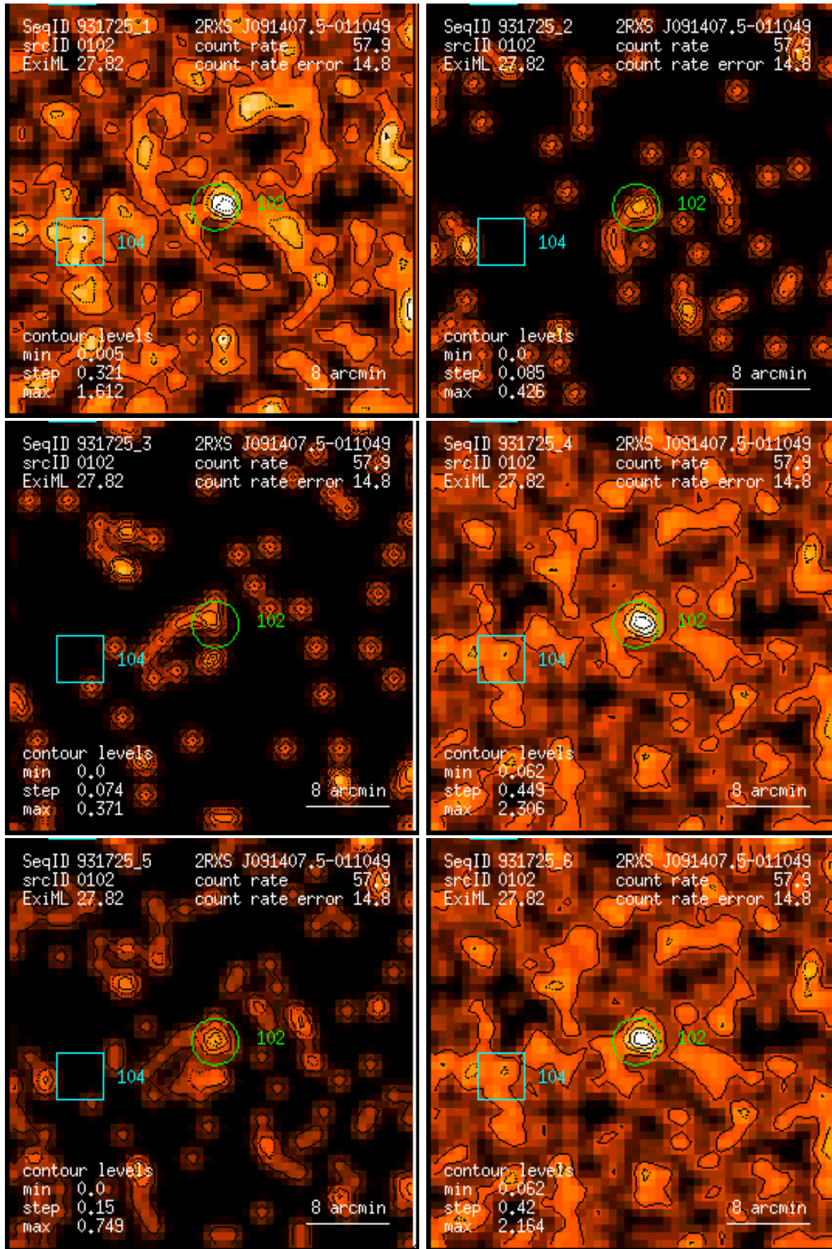
Figure 102: RASS 931725: detection 0102: band rate images, Gaussian filter: (1) PSPC channels 11 – 41, (2) 52 – 90, (3) 91 – 201, (4) 11 – 235, (5) 52 – 201, (6) 11 – 201. Broad band rates in counts/ks. Band rate contour levels in counts/ks/arcmin 2 .
