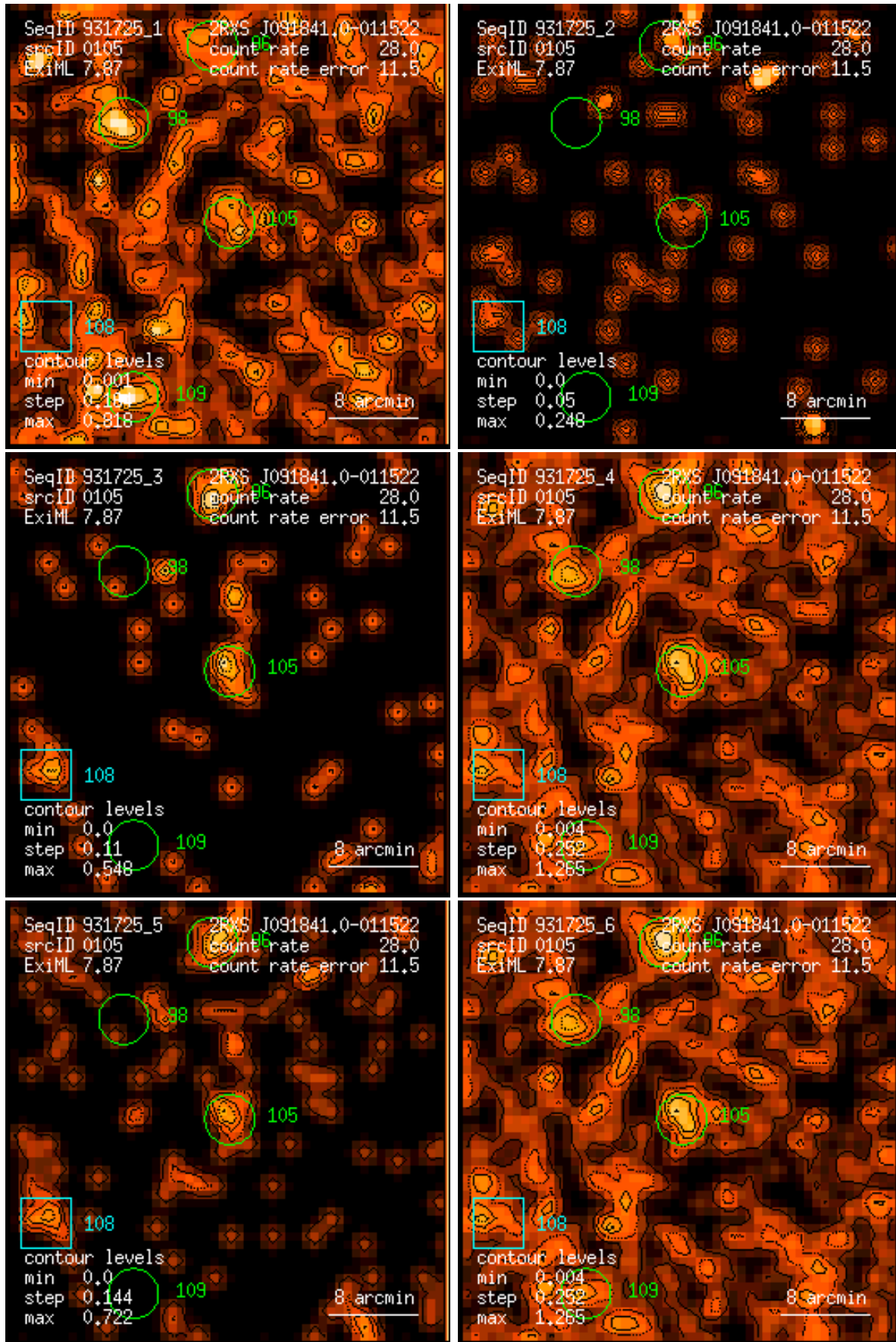
Figure 105: RASS 931725: detection 0105: band rate images, Gaussian filter: (1) PSPC channels 11 – 41, (2) 52 – 90, (3) 91 – 201, (4) 11 – 235, (5) 52 – 201, (6) 11 – 201. Broad band rates in counts/ks. Band rate contour levels in counts/ks/arcmin 2 .
