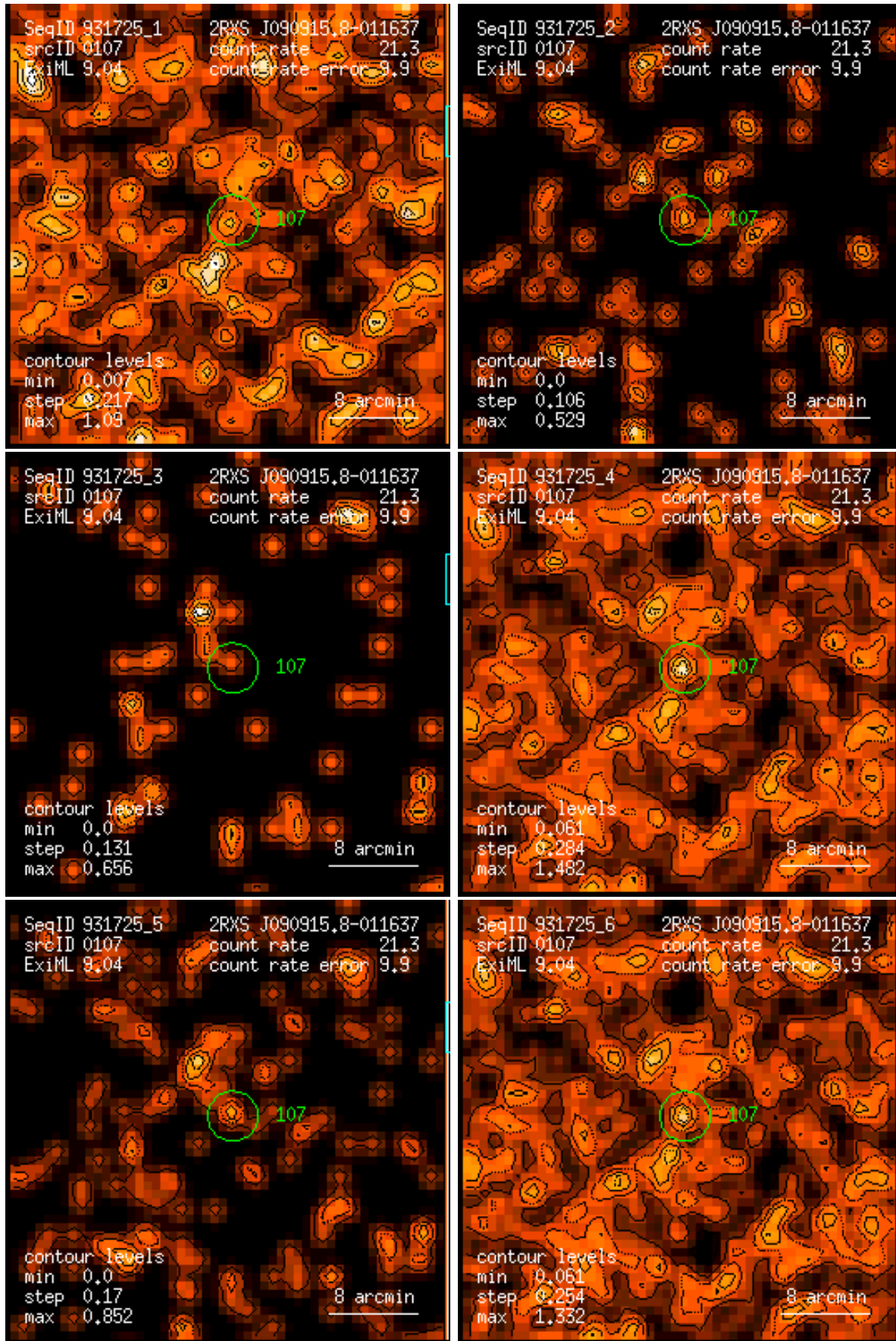
Figure 107: RASS 931725: detection 0107: band rate images, Gaussian filter: (1) PSPC channels 11 – 41, (2) 52 – 90, (3) 91 – 201, (4) 11 – 235, (5) 52 – 201, (6) 11 – 201. Broad band rates in counts/ks. Band rate contour levels in counts/ks/arcmin 2 .
