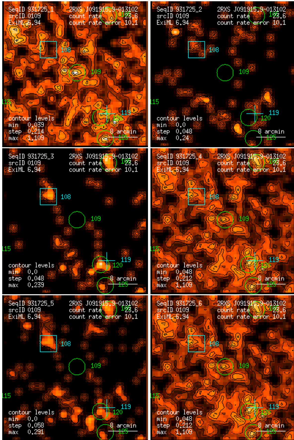
Figure 109: RASS 931725: detection 0109: band rate images, Gaussian filter: (1) PSPC channels 11 – 41, (2) 52 – 90, (3) 91 – 201, (4) 11 – 235, (5) 52 – 201, (6) 11 – 201. Broad band rates in counts/ks. Band rate contour levels in counts/ks/arcmin 2 .
