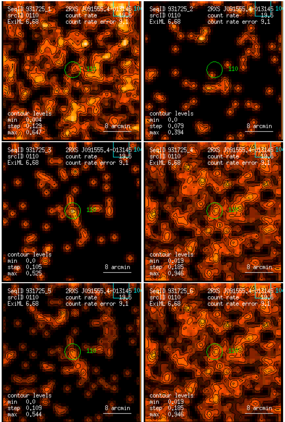
Figure 110: RASS 931725: detection 0110: band rate images, Gaussian filter: (1) PSPC channels 11 – 41, (2) 52 – 90, (3) 91 – 201, (4) 11 – 235, (5) 52 – 201, (6) 11 – 201. Broad band rates in counts/ks. Band rate contour levels in counts/ks/arcmin 2 .
