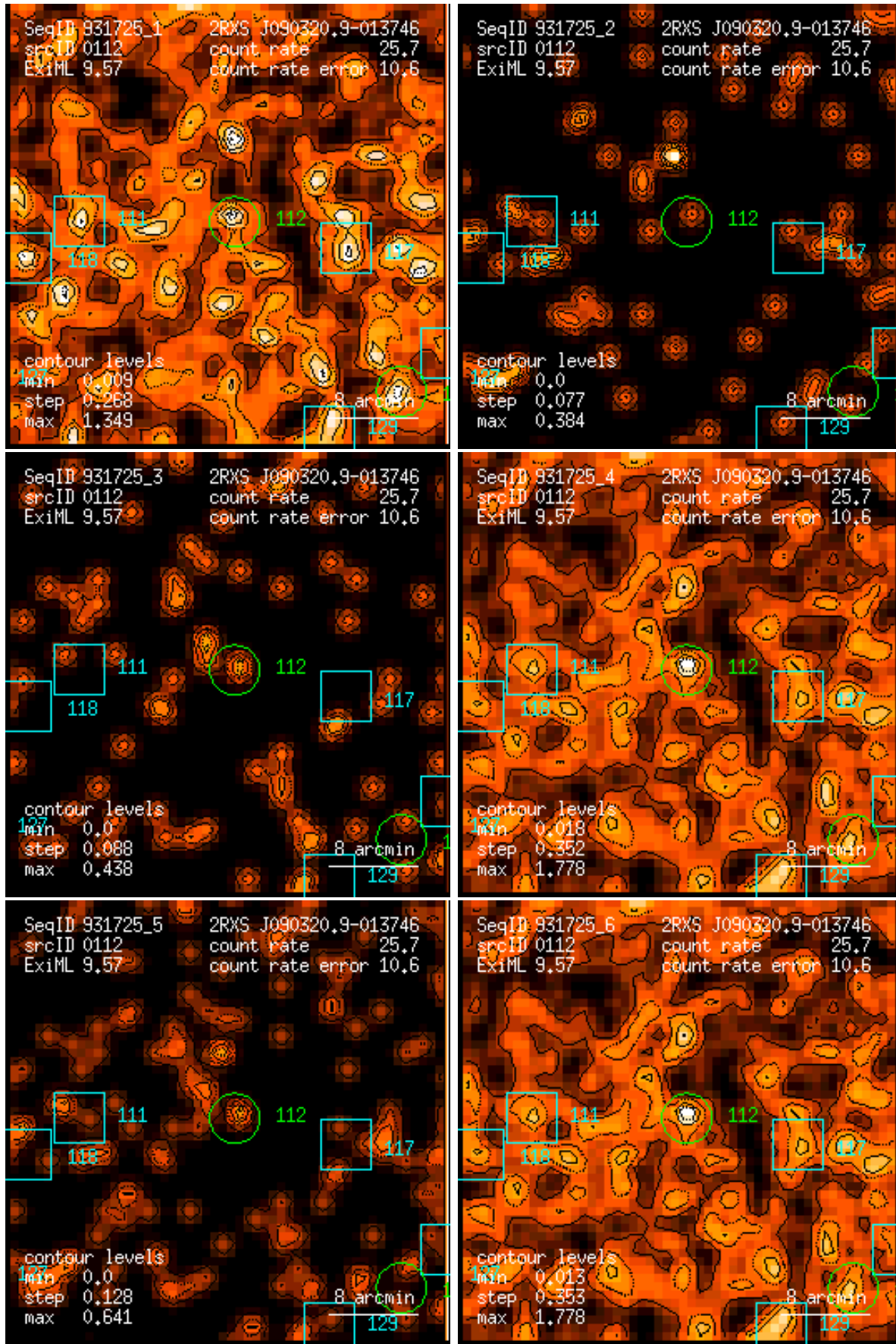
Figure 112: RASS 931725: detection 0112: band rate images, Gaussian filter: (1) PSPC channels 11 – 41, (2) 52 – 90, (3) 91 – 201, (4) 11 – 235, (5) 52 – 201, (6) 11 – 201. Broad band rates in counts/ks. Band rate contour levels in counts/ks/arcmin 2 .
