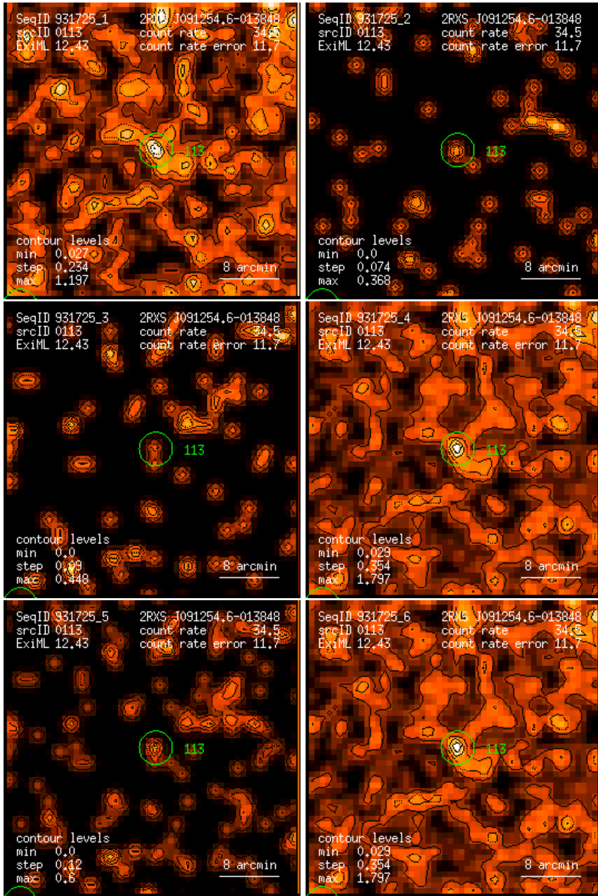
Figure 113: RASS 931725: detection 0113: band rate images, Gaussian filter: (1) PSPC channels 11 – 41, (2) 52 – 90, (3) 91 – 201, (4) 11 – 235, (5) 52 – 201, (6) 11 – 201. Broad band rates in counts/ks. Band rate contour levels in counts/ks/arcmin 2 .
