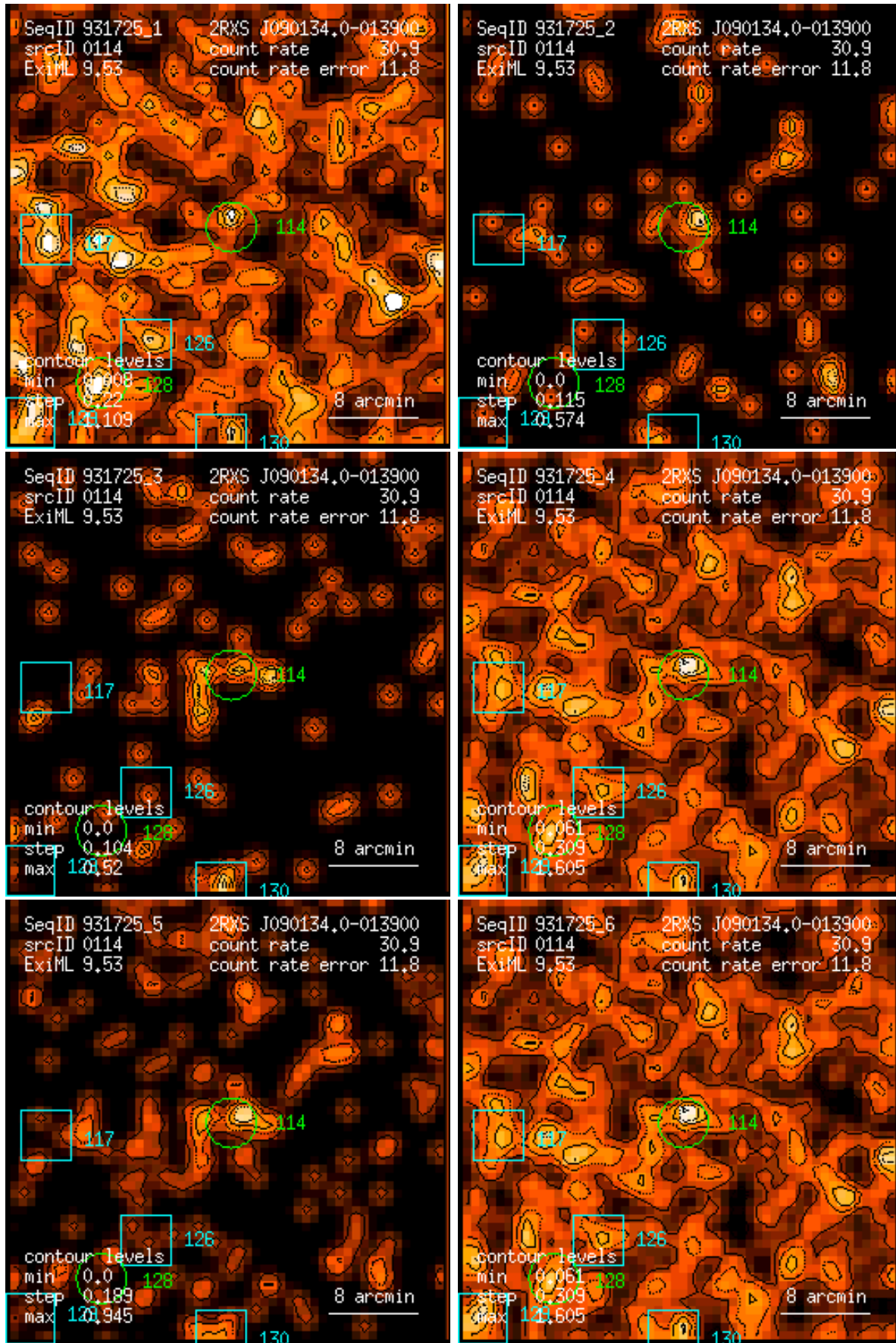
Figure 114: RASS 931725: detection 0114: band rate images, Gaussian filter: (1) PSPC channels 11 – 41, (2) 52 – 90, (3) 91 – 201, (4) 11 – 235, (5) 52 – 201, (6) 11 – 201. Broad band rates in counts/ks. Band rate contour levels in counts/ks/arcmin 2 .
