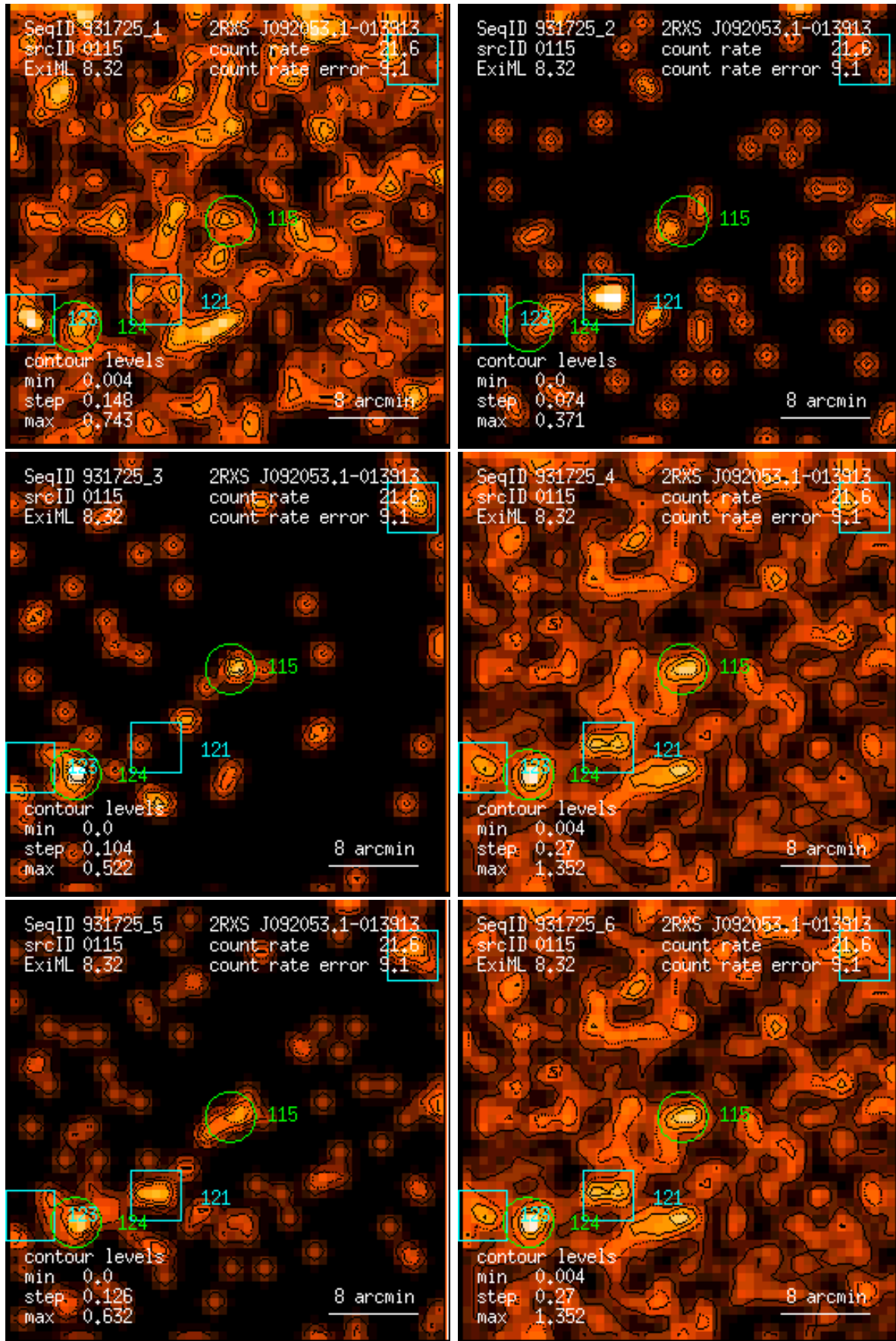
Figure 115: RASS 931725: detection 0115: band rate images, Gaussian filter: (1) PSPC channels 11 – 41, (2) 52 – 90, (3) 91 – 201, (4) 11 – 235, (5) 52 – 201, (6) 11 – 201. Broad band rates in counts/ks. Band rate contour levels in counts/ks/arcmin 2 .
