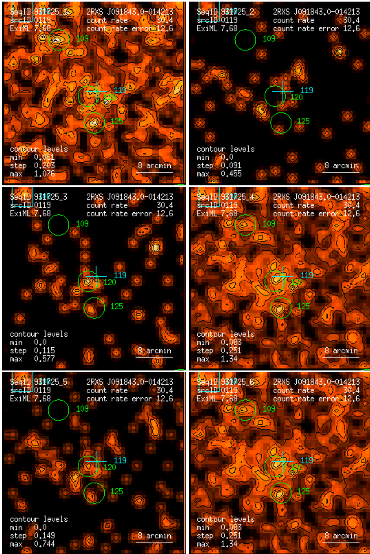
Figure 119: RASS 931725: detection 0119: band rate images, Gaussian filter: (1) PSPC channels 11 – 41, (2) 52 – 90, (3) 91 – 201, (4) 11 – 235, (5) 52 – 201, (6) 11 – 201. Broad band rates in counts/ks. Band rate contour levels in counts/ks/arcmin 2 .
