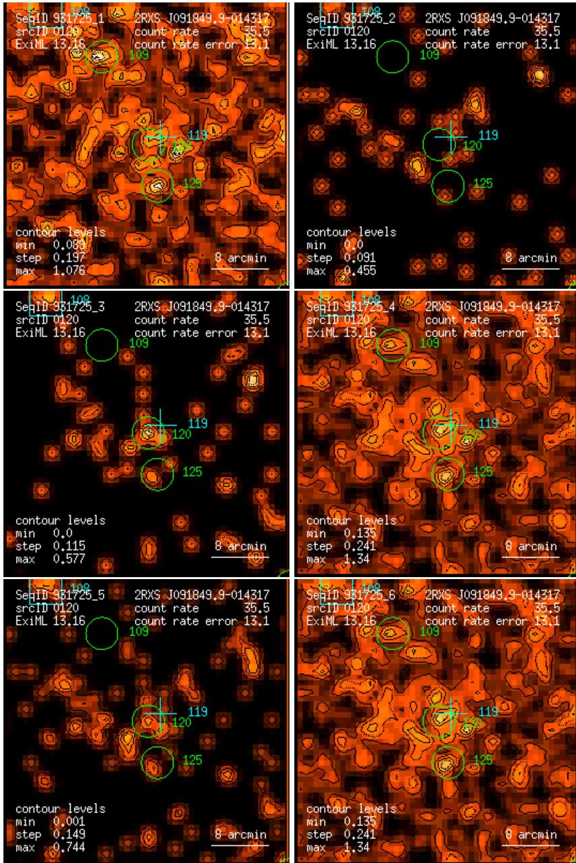
Figure 120: RASS 931725: detection 0120: band rate images, Gaussian filter: (1) PSPC channels 11 – 41, (2) 52 – 90, (3) 91 – 201, (4) 11 – 235, (5) 52 – 201, (6) 11 – 201. Broad band rates in counts/ks. Band rate contour levels in counts/ks/arcmin 2 .
