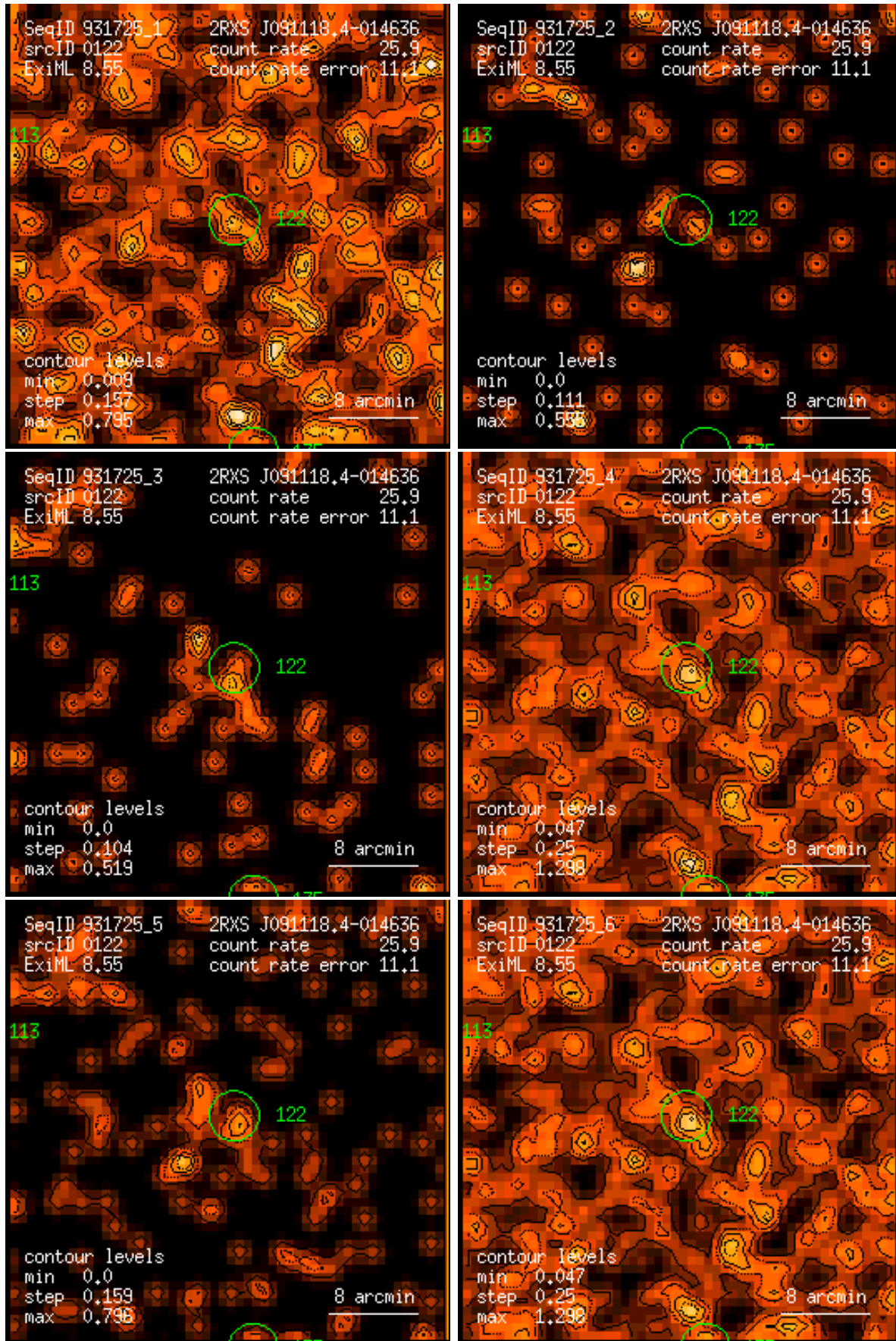
Figure 122: RASS 931725: detection 0122: band rate images, Gaussian filter: (1) PSPC channels 11 – 41, (2) 52 – 90, (3) 91 – 201, (4) 11 – 235, (5) 52 – 201, (6) 11 – 201. Broad band rates in counts/ks. Band rate contour levels in counts/ks/arcmin 2 .
