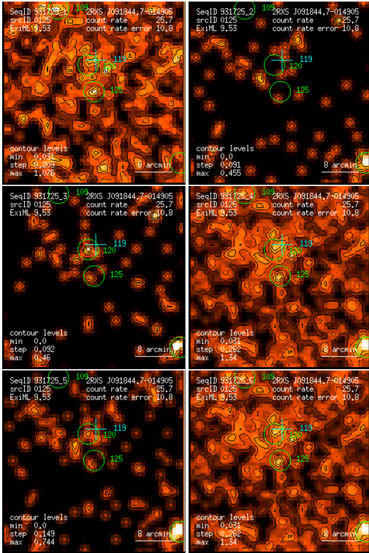
Figure 125: RASS 931725: detection 0125: band rate images, Gaussian filter: (1) PSPC channels 11 – 41, (2) 52 – 90, (3) 91 – 201, (4) 11 – 235, (5) 52 – 201, (6) 11 – 201. Broad band rates in counts/ks. Band rate contour levels in counts/ks/arcmin 2 .
