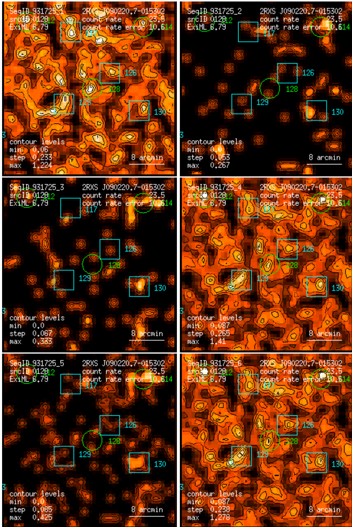
Figure 128: RASS 931725: detection 0128: band rate images, Gaussian filter: (1) PSPC channels 11 – 41, (2) 52 – 90, (3) 91 – 201, (4) 11 – 235, (5) 52 – 201, (6) 11 – 201. Broad band rates in counts/ks. Band rate contour levels in counts/ks/arcmin 2 .
