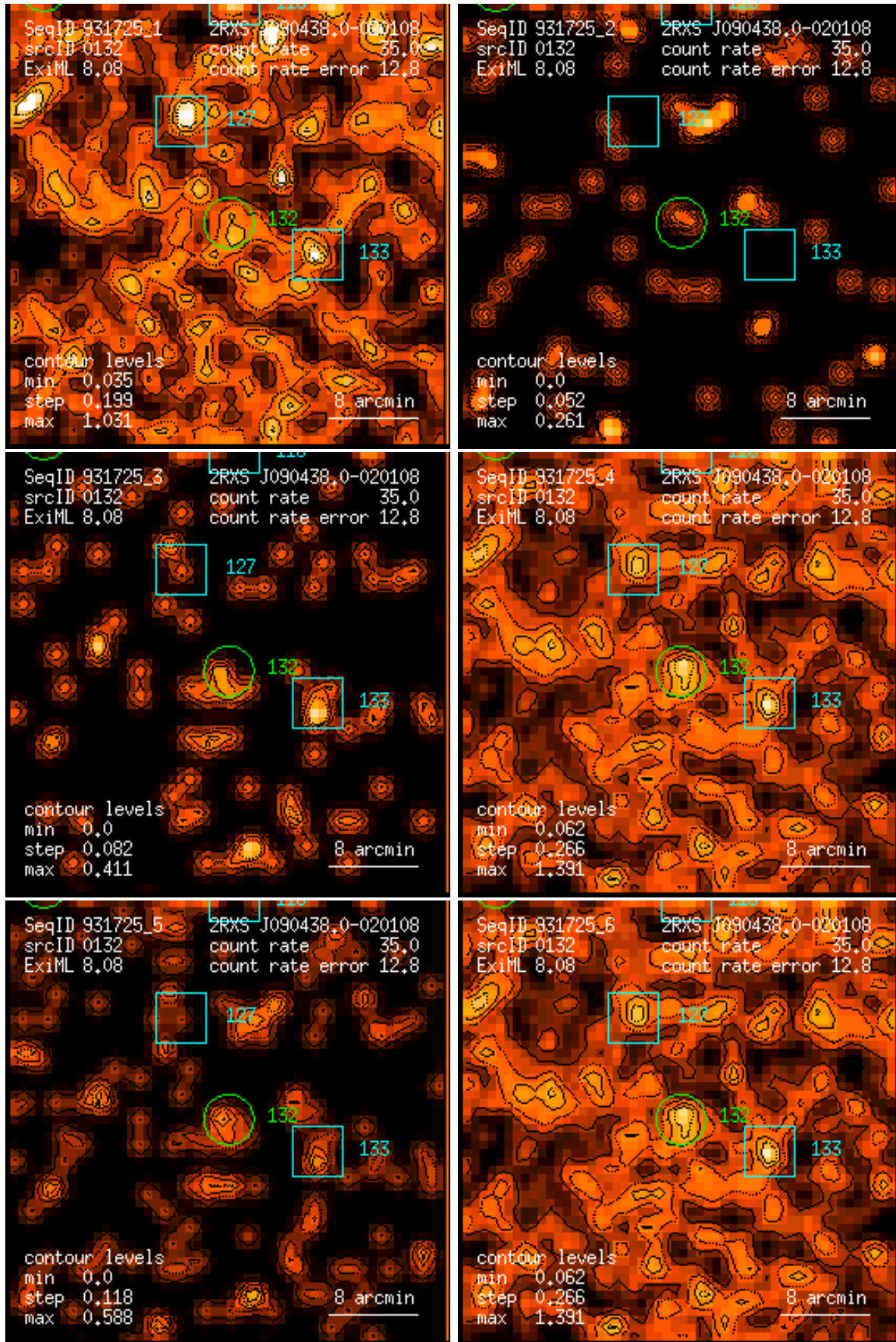
Figure 132: RASS 931725: detection 0132: band rate images, Gaussian filter: (1) PSPC channels 11 – 41, (2) 52 – 90, (3) 91 – 201, (4) 11 – 235, (5) 52 – 201, (6) 11 – 201. Broad band rates in counts/ks. Band rate contour levels in counts/ks/arcmin 2 .
