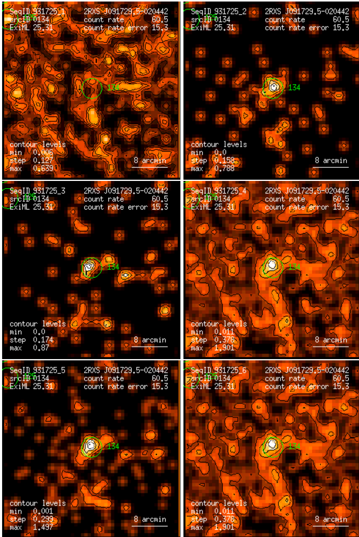
Figure 134: RASS 931725: detection 0134: band rate images, Gaussian filter: (1) PSPC channels 11 – 41, (2) 52 – 90, (3) 91 – 201, (4) 11 – 235, (5) 52 – 201, (6) 11 – 201. Broad band rates in counts/ks. Band rate contour levels in counts/ks/arcmin 2 .
