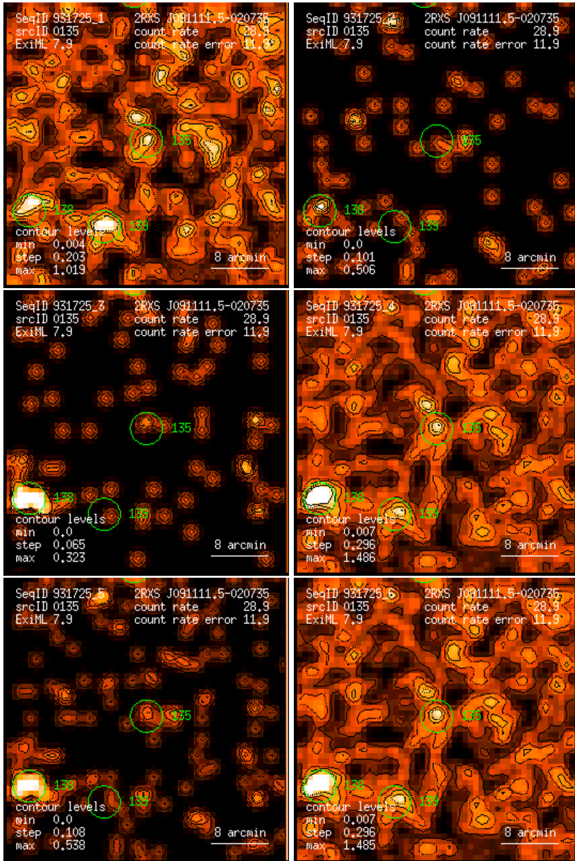
Figure 135: RASS 931725: detection 0135: band rate images, Gaussian filter: (1) PSPC channels 11 – 41, (2) 52 – 90, (3) 91 – 201, (4) 11 – 235, (5) 52 – 201, (6) 11 – 201. Broad band rates in counts/ks. Band rate contour levels in counts/ks/arcmin 2 .
