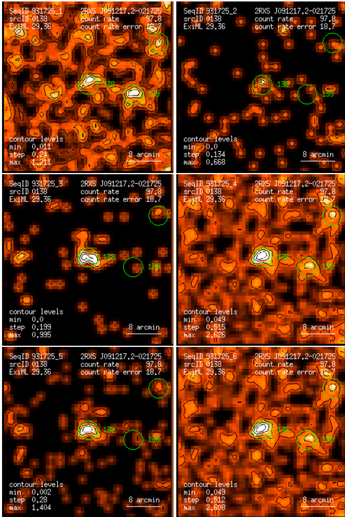
Figure 138: RASS 931725: detection 0138: band rate images, Gaussian filter: (1) PSPC channels 11 – 41, (2) 52 – 90, (3) 91 – 201, (4) 11 – 235, (5) 52 – 201, (6) 11 – 201. Broad band rates in counts/ks. Band rate contour levels in counts/ks/arcmin 2 .
