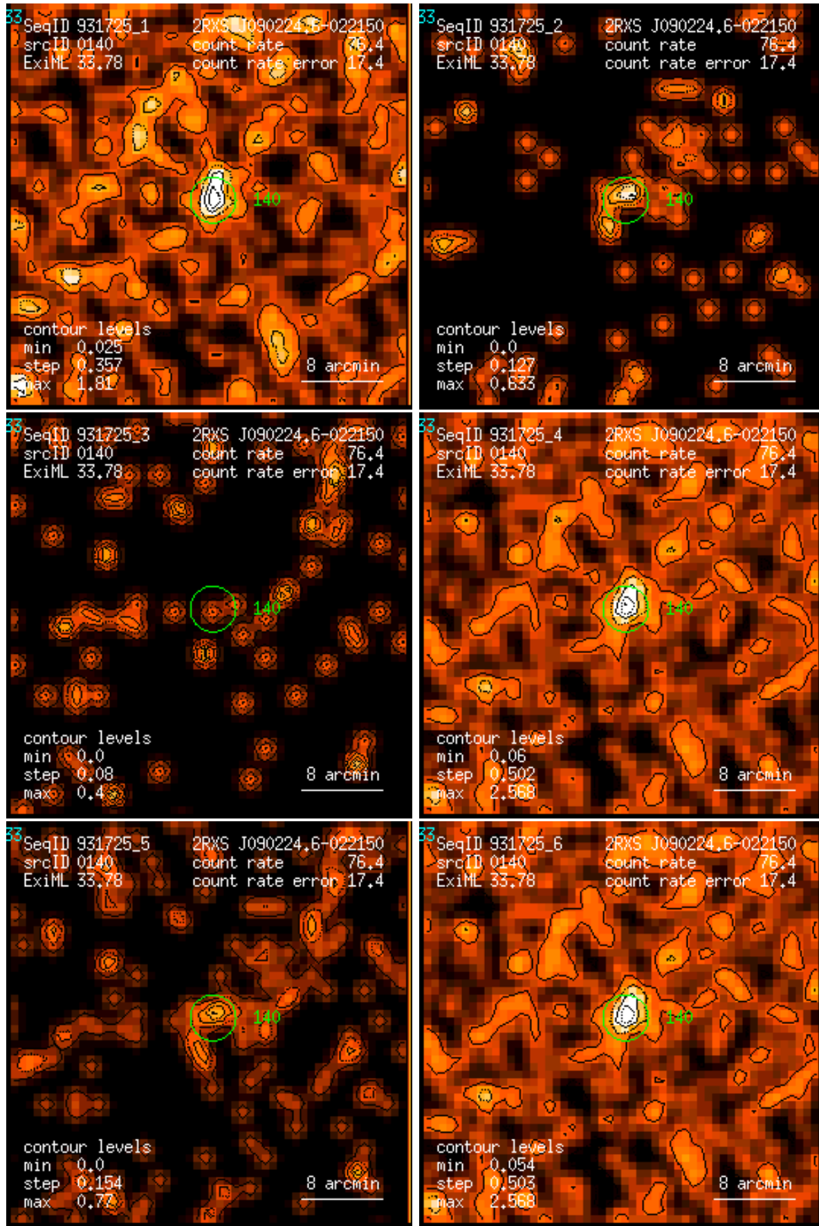
Figure 140: RASS 931725: detection 0140: band rate images, Gaussian filter: (1) PSPC channels 11 – 41, (2) 52 – 90, (3) 91 – 201, (4) 11 – 235, (5) 52 – 201, (6) 11 – 201. Broad band rates in counts/ks. Band rate contour levels in counts/ks/arcmin 2 .
