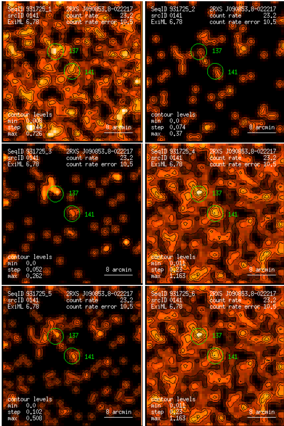
Figure 141: RASS 931725: detection 0141: band rate images, Gaussian filter: (1) PSPC channels 11 – 41, (2) 52 – 90, (3) 91 – 201, (4) 11 – 235, (5) 52 – 201, (6) 11 – 201. Broad band rates in counts/ks. Band rate contour levels in counts/ks/arcmin 2 .
