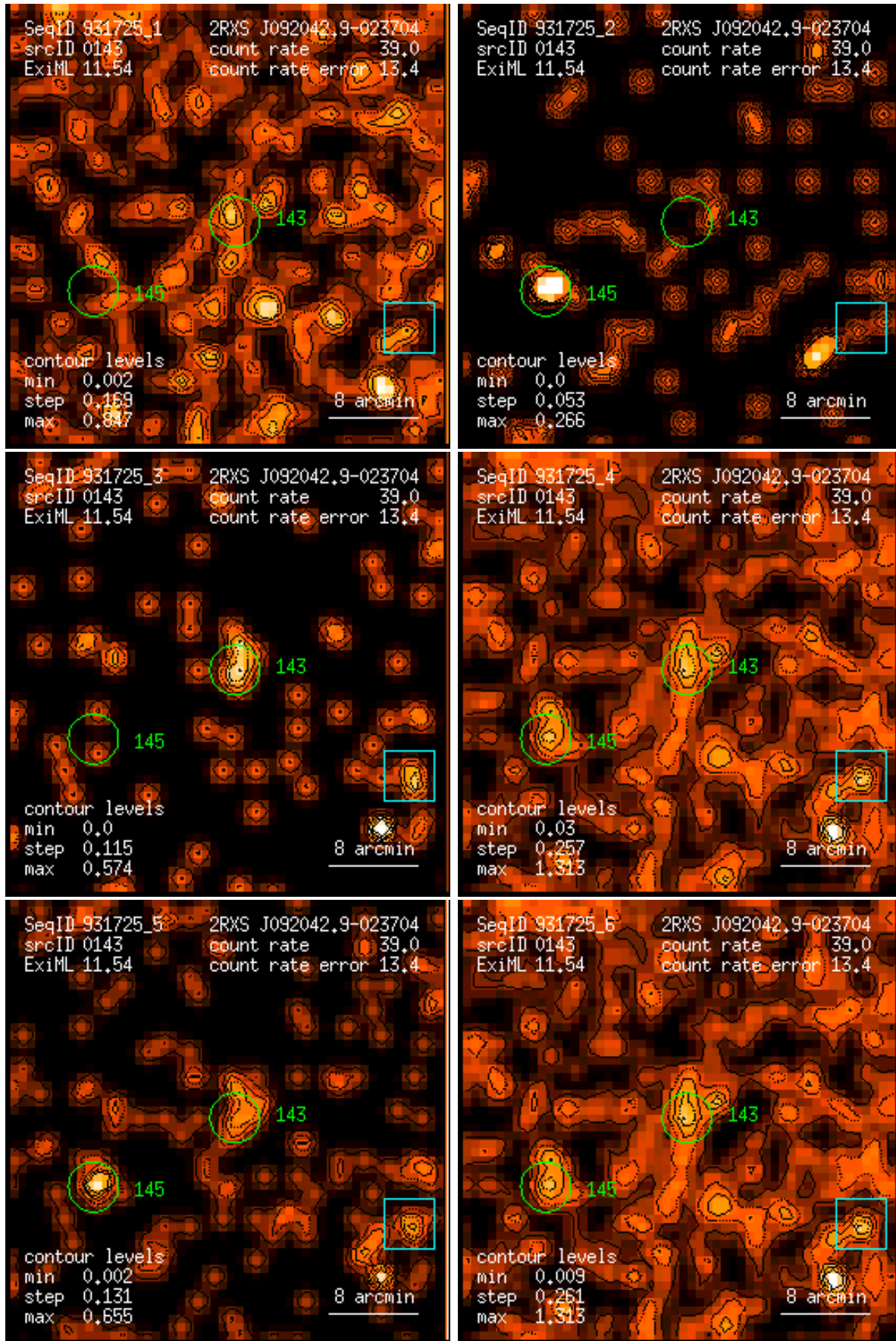
Figure 143: RASS 931725: detection 0143: band rate images, Gaussian filter: (1) PSPC channels 11 – 41, (2) 52 – 90, (3) 91 – 201, (4) 11 – 235, (5) 52 – 201, (6) 11 – 201. Broad band rates in counts/ks. Band rate contour levels in counts/ks/arcmin 2 .
