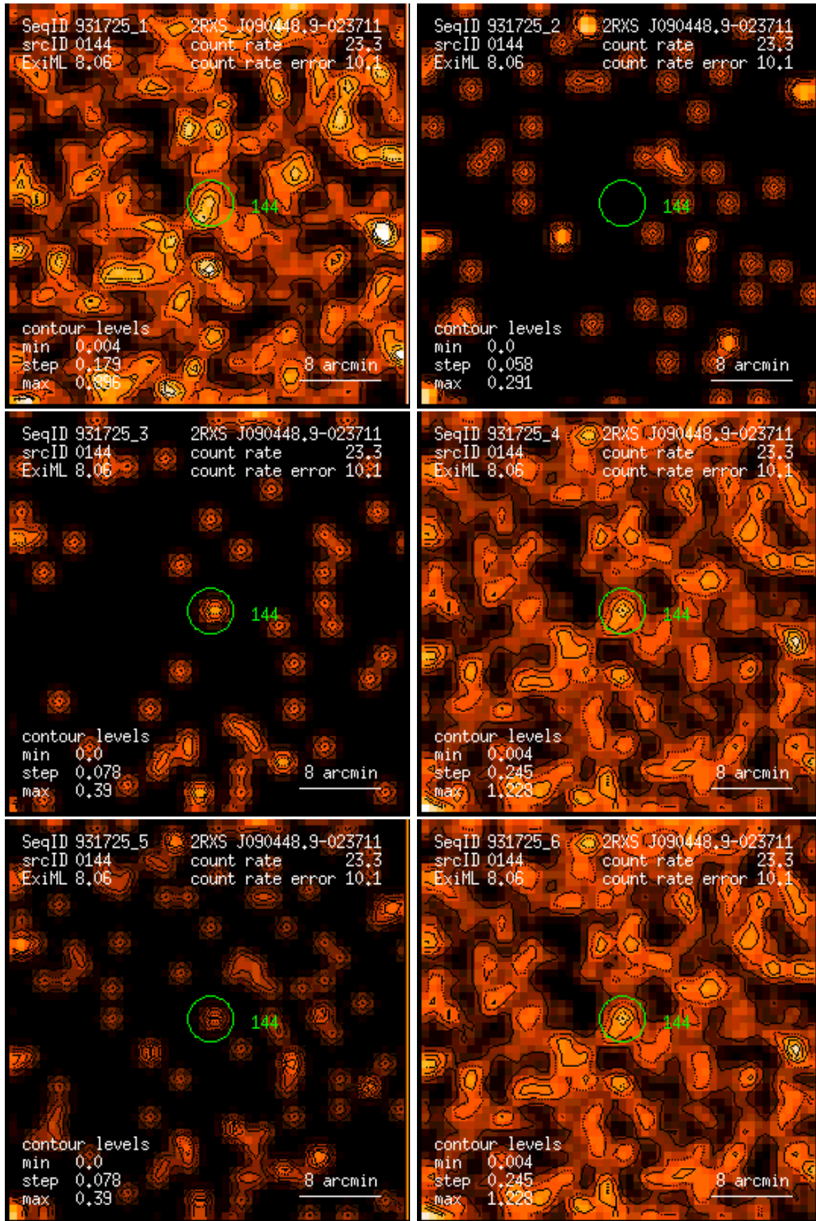
Figure 144: RASS 931725: detection 0144: band rate images, Gaussian filter: (1) PSPC channels 11 – 41, (2) 52 – 90, (3) 91 – 201, (4) 11 – 235, (5) 52 – 201, (6) 11 – 201. Broad band rates in counts/ks. Band rate contour levels in counts/ks/arcmin 2 .
