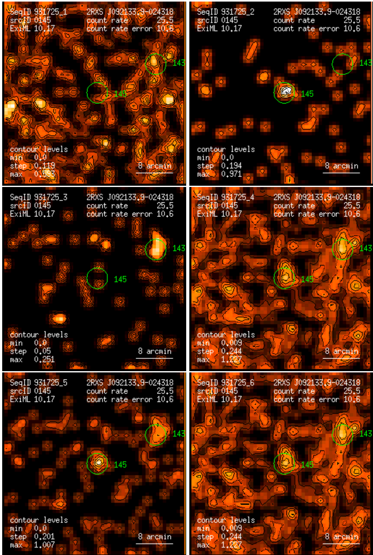
Figure 145: RASS 931725: detection 0145: band rate images, Gaussian filter: (1) PSPC channels 11 – 41, (2) 52 – 90, (3) 91 – 201, (4) 11 – 235, (5) 52 – 201, (6) 11 – 201. Broad band rates in counts/ks. Band rate contour levels in counts/ks/arcmin 2 .
