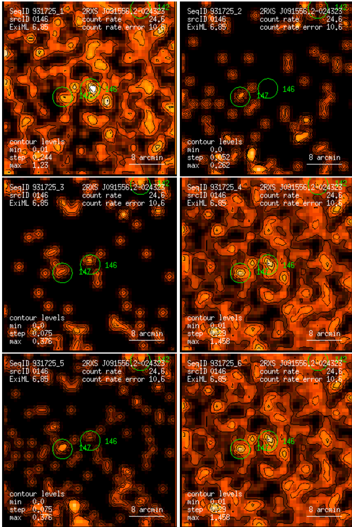
Figure 146: RASS 931725: detection 0146: band rate images, Gaussian filter: (1) PSPC channels 11 – 41, (2) 52 – 90, (3) 91 – 201, (4) 11 – 235, (5) 52 – 201, (6) 11 – 201. Broad band rates in counts/ks. Band rate contour levels in counts/ks/arcmin 2 .
