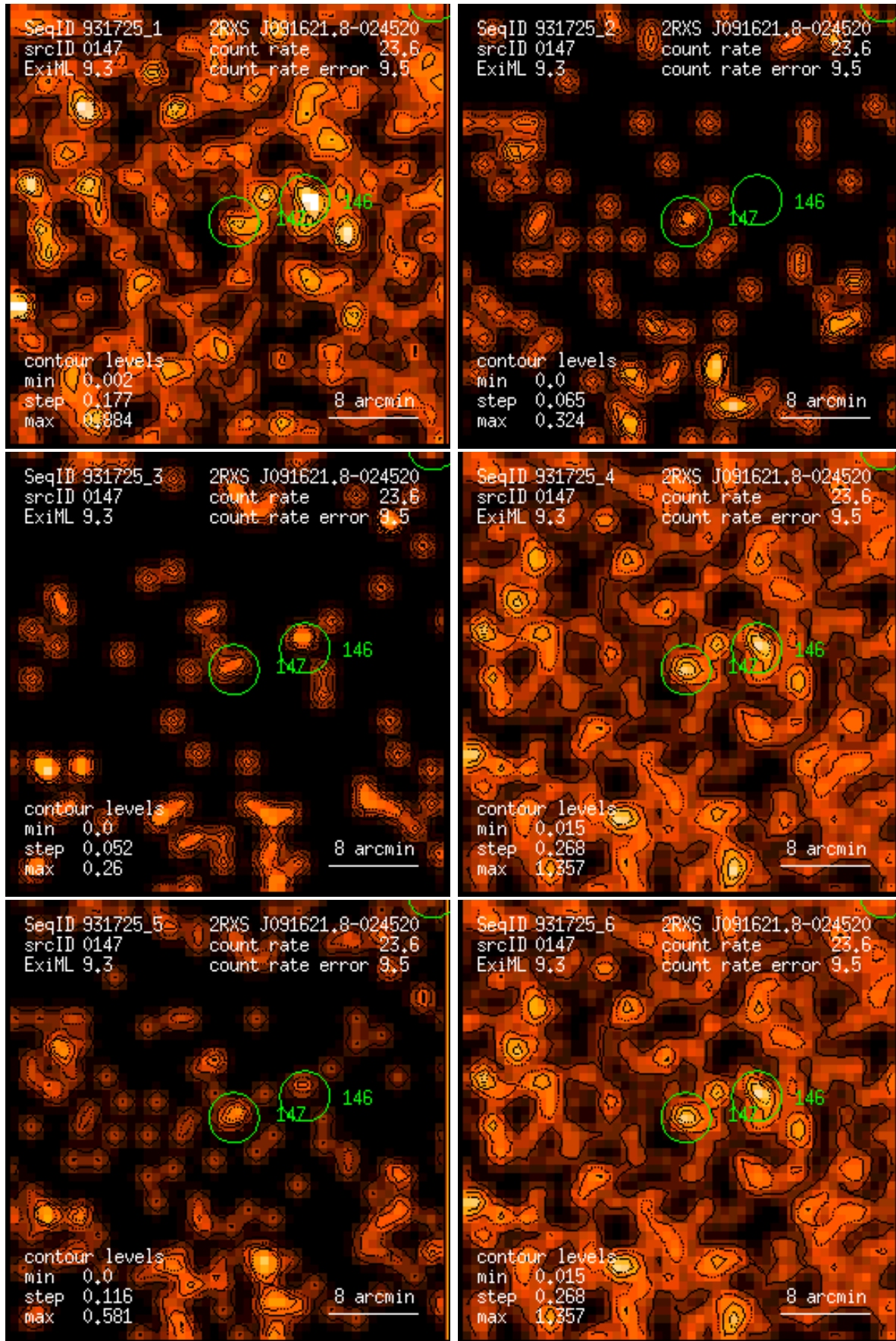
Figure 147: RASS 931725: detection 0147: band rate images, Gaussian filter: (1) PSPC channels 11 – 41, (2) 52 – 90, (3) 91 – 201, (4) 11 – 235, (5) 52 – 201, (6) 11 – 201. Broad band rates in counts/ks. Band rate contour levels in counts/ks/arcmin 2 .
