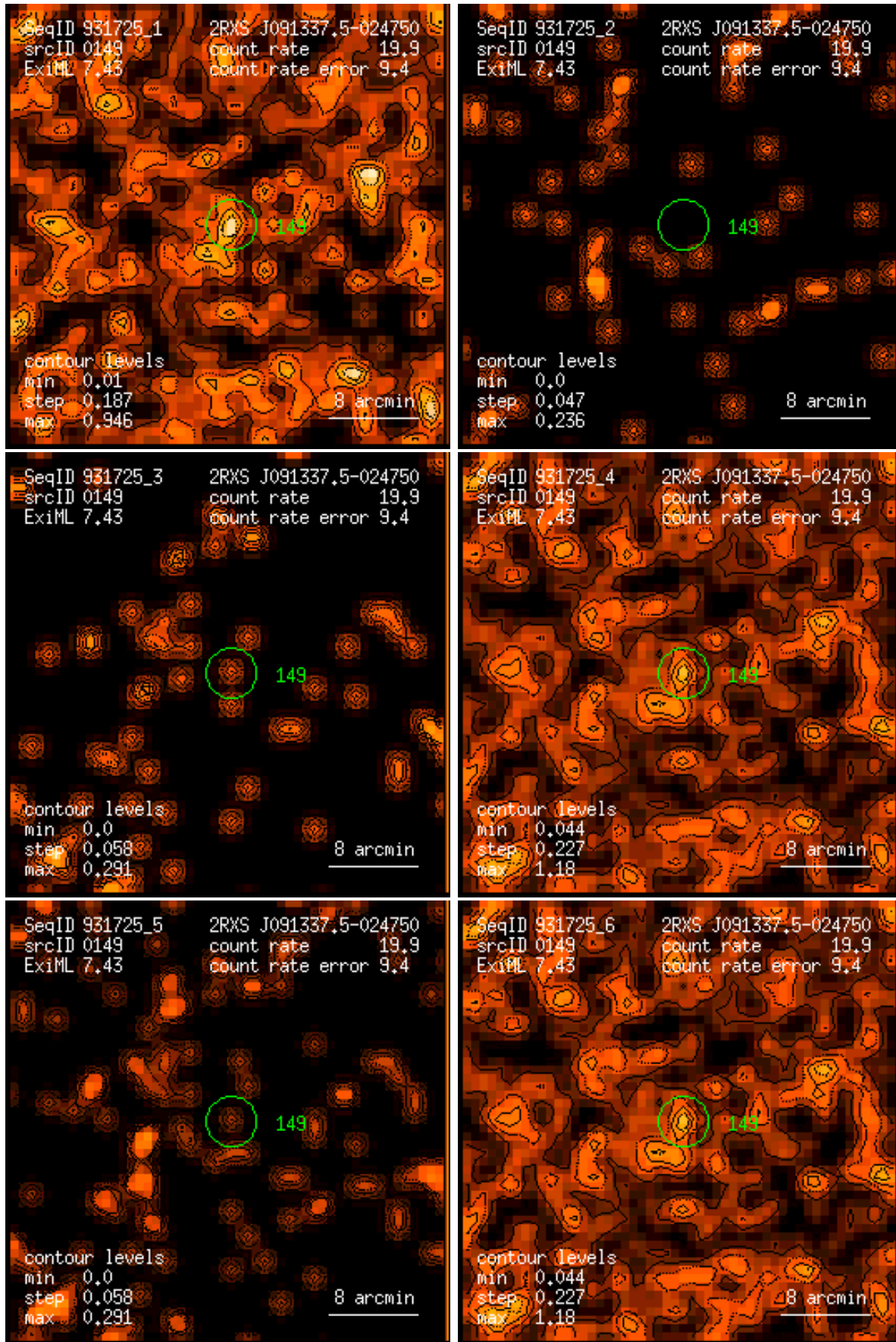
Figure 149: RASS 931725: detection 0149: band rate images, Gaussian filter: (1) PSPC channels 11 – 41, (2) 52 – 90, (3) 91 – 201, (4) 11 – 235, (5) 52 – 201, (6) 11 – 201. Broad band rates in counts/ks. Band rate contour levels in counts/ks/arcmin 2 .
