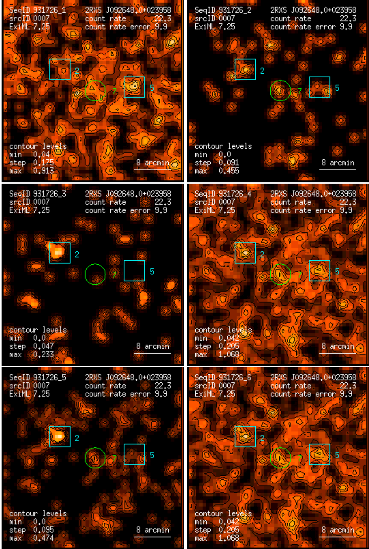
Figure 7: RASS 931726: detection 0007: band rate images, Gaussian filter: (1) PSPC channels 11 – 41, (2) 52 – 90, (3) 91 – 201, (4) 11 – 235, (5) 52 – 201, (6) 11 – 201. Broad band rates in counts/ks. Band rate contour levels in counts/ks/arcmin 2 .
