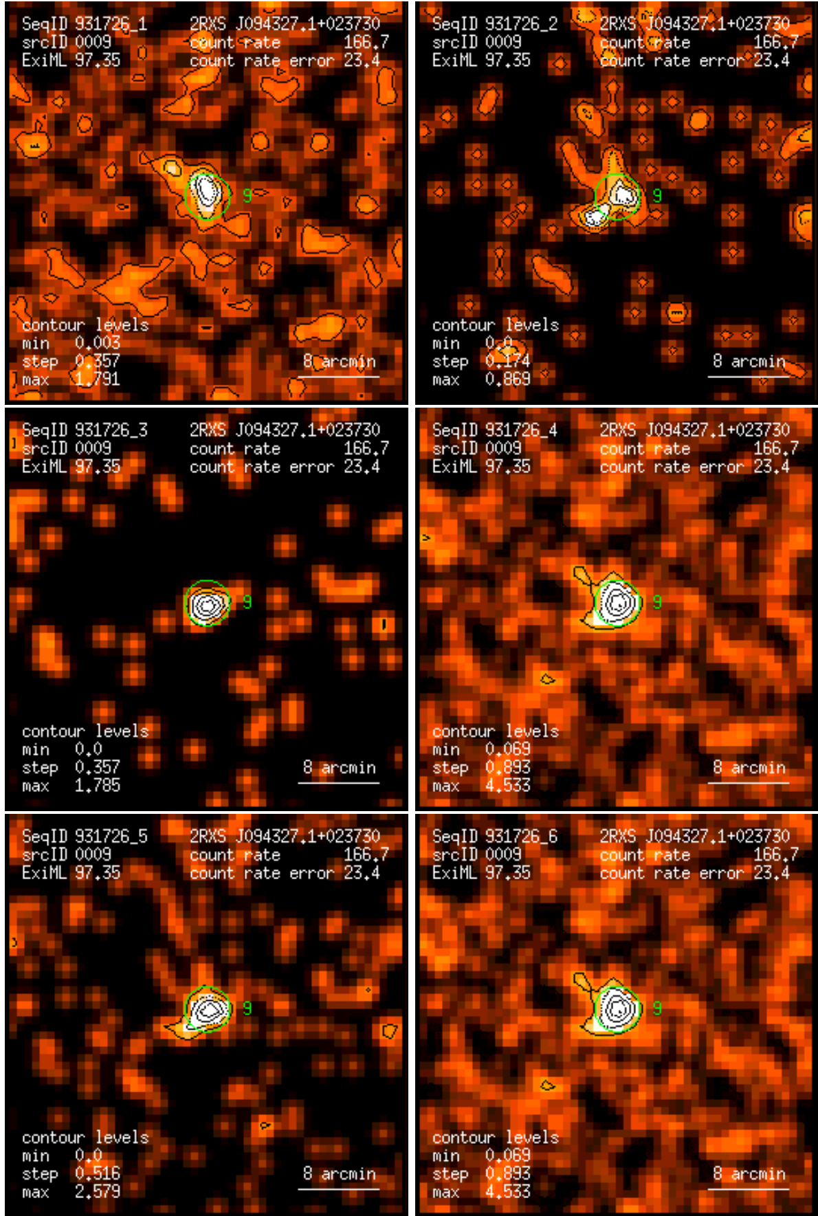
Figure 9: RASS 931726: detection 0009: band rate images, Gaussian filter: (1) PSPC channels 11 – 41, (2) 52 – 90, (3) 91 – 201, (4) 11 – 235, (5) 52 – 201, (6) 11 – 201. Broad band rates in counts/ks. Band rate contour levels in counts/ks/arcmin 2 .
