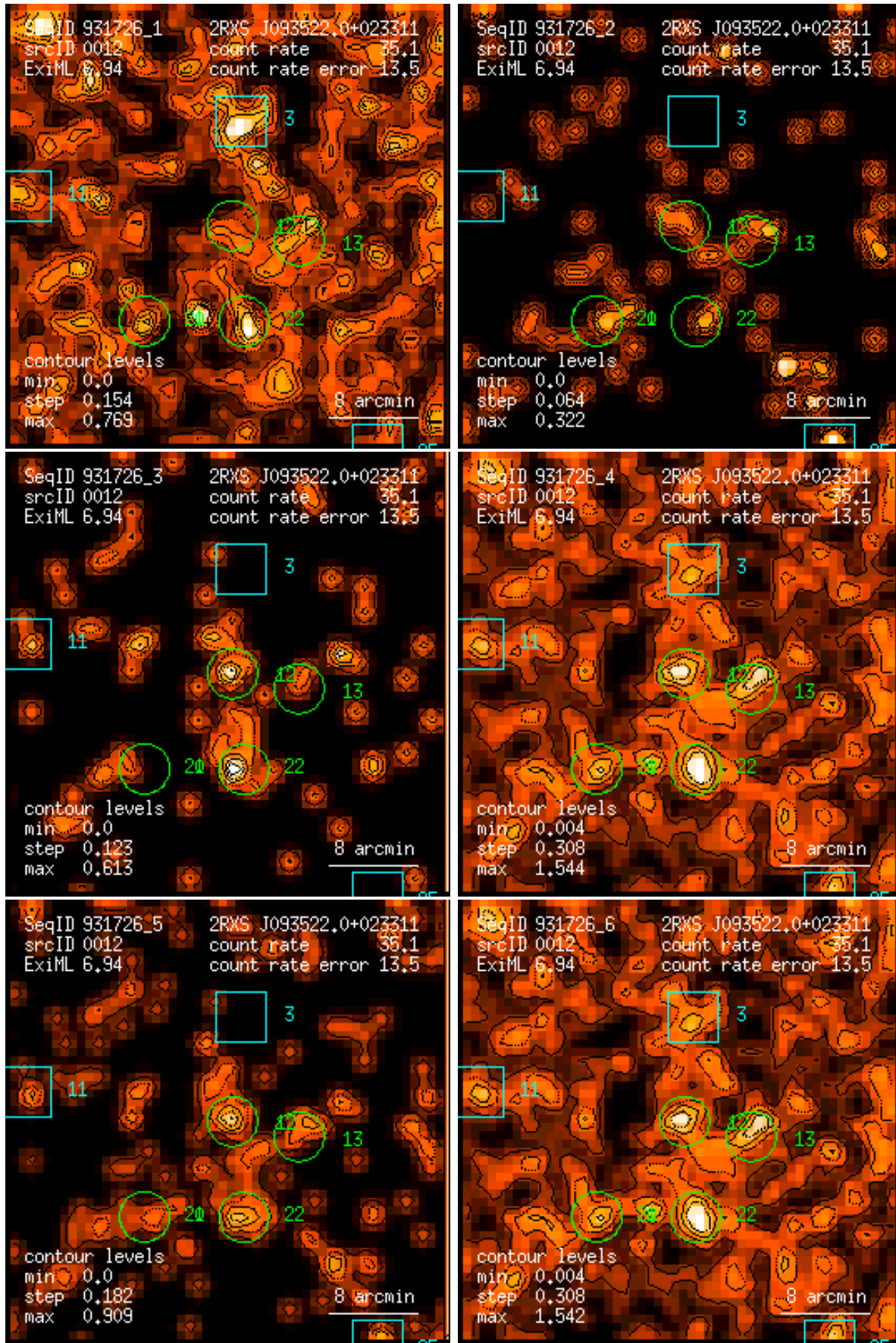
Figure 12: RASS 931726: detection 0012: band rate images, Gaussian filter: (1) PSPC channels 11 – 41, (2) 52 – 90, (3) 91 – 201, (4) 11 – 235, (5) 52 – 201, (6) 11 – 201. Broad band rates in counts/ks. Band rate contour levels in counts/ks/arcmin 2 .
