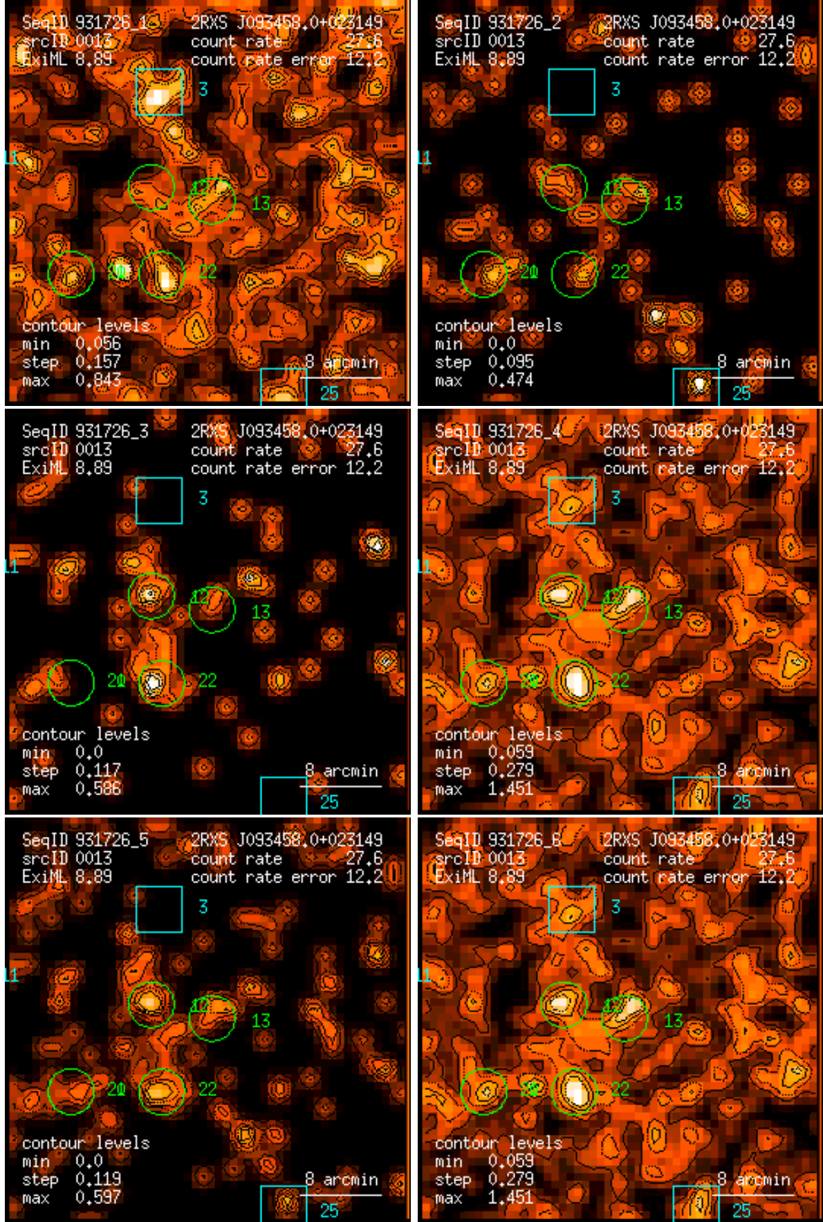
Figure 13: RASS 931726: detection 0013: band rate images, Gaussian filter: (1) PSPC channels 11 – 41, (2) 52 – 90, (3) 91 – 201, (4) 11 – 235, (5) 52 – 201, (6) 11 – 201. Broad band rates in counts/ks. Band rate contour levels in counts/ks/arcmin 2 .
