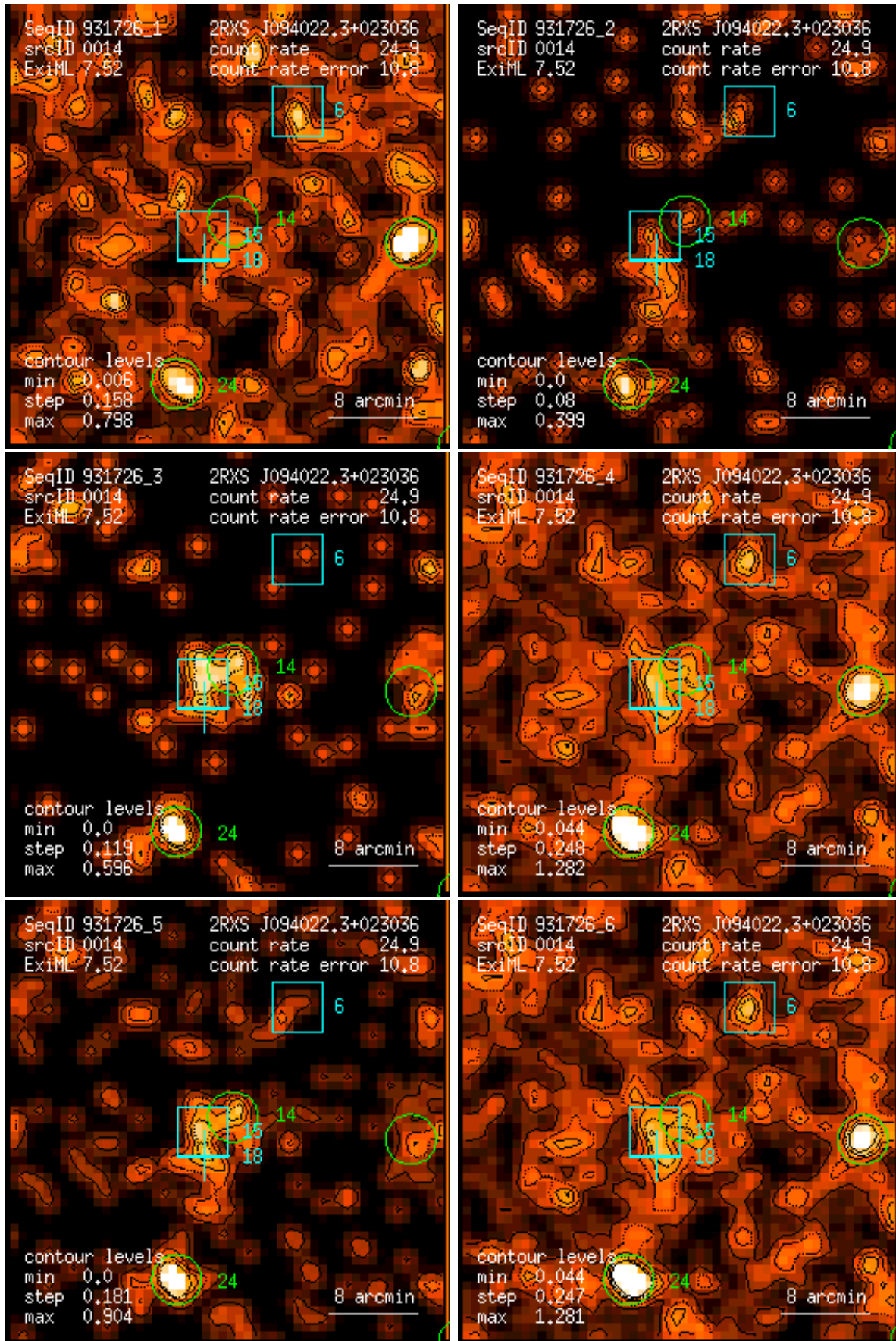
Figure 14: RASS 931726: detection 0014: band rate images, Gaussian filter: (1) PSPC channels 11 – 41, (2) 52 – 90, (3) 91 – 201, (4) 11 – 235, (5) 52 – 201, (6) 11 – 201. Broad band rates in counts/ks. Band rate contour levels in counts/ks/arcmin 2 .
