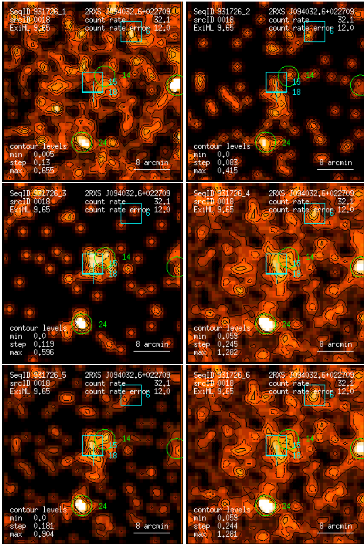
Figure 18: RASS 931726: detection 0018: band rate images, Gaussian filter: (1) PSPC channels 11 – 41, (2) 52 – 90, (3) 91 – 201, (4) 11 – 235, (5) 52 – 201, (6) 11 – 201. Broad band rates in counts/ks. Band rate contour levels in counts/ks/arcmin 2 .
