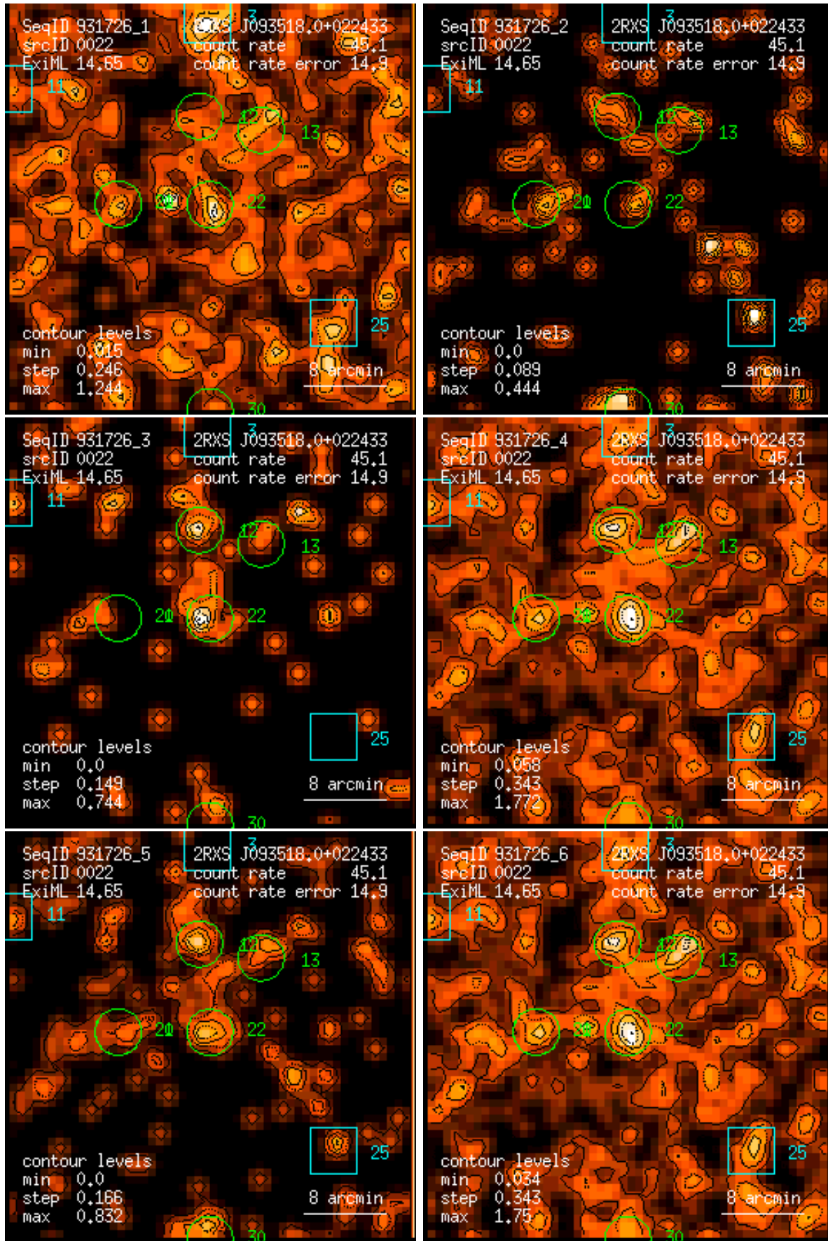
Figure 22: RASS 931726: detection 0022: band rate images, Gaussian filter: (1) PSPC channels 11 – 41, (2) 52 – 90, (3) 91 – 201, (4) 11 – 235, (5) 52 – 201, (6) 11 – 201. Broad band rates in counts/ks. Band rate contour levels in counts/ks/arcmin 2 .
