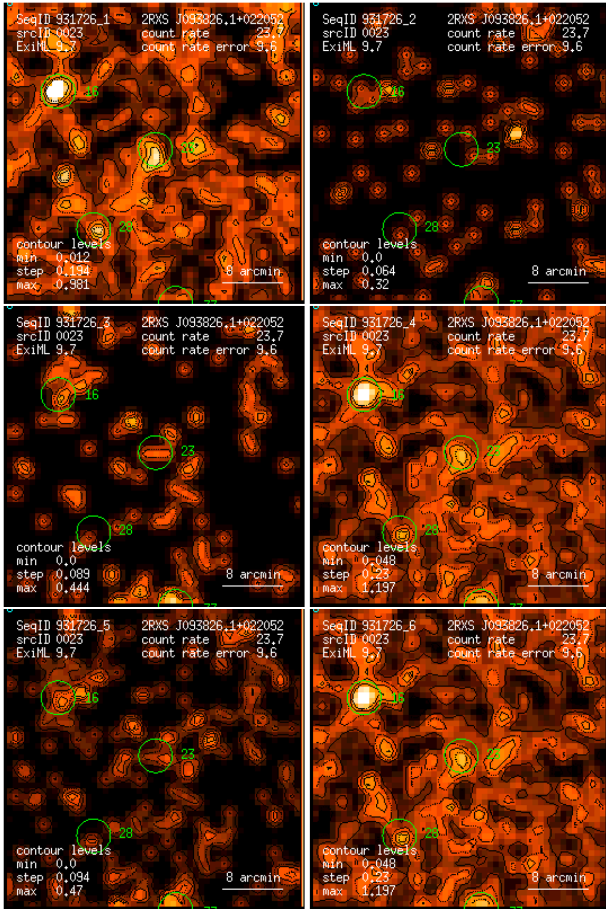
Figure 23: RASS 931726: detection 0023: band rate images, Gaussian filter: (1) PSPC channels 11 – 41, (2) 52 – 90, (3) 91 – 201, (4) 11 – 235, (5) 52 – 201, (6) 11 – 201. Broad band rates in counts/ks. Band rate contour levels in counts/ks/arcmin 2 .
