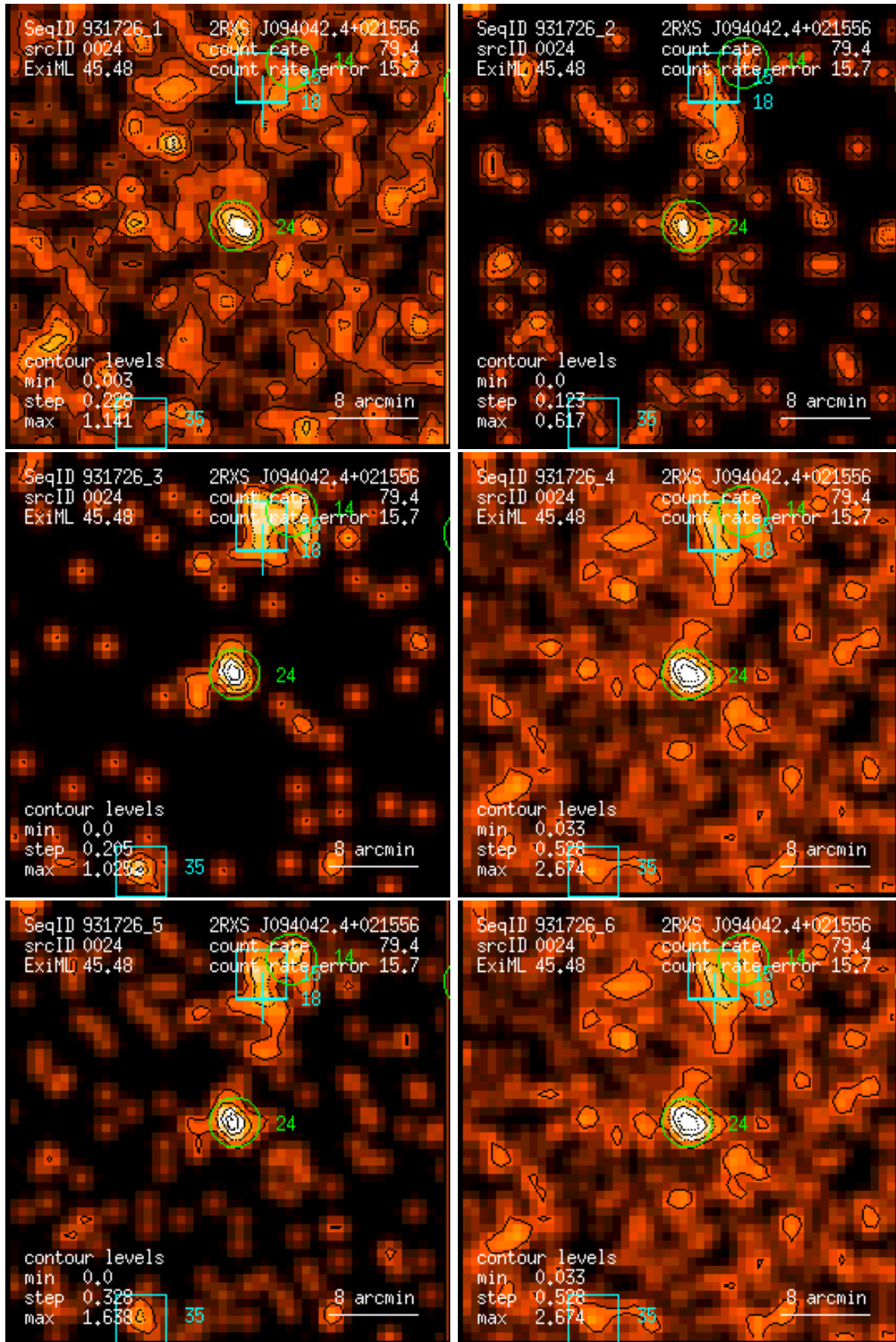
Figure 24: RASS 931726: detection 0024: band rate images, Gaussian filter: (1) PSPC channels 11 – 41, (2) 52 – 90, (3) 91 – 201, (4) 11 – 235, (5) 52 – 201, (6) 11 – 201. Broad band rates in counts/ks. Band rate contour levels in counts/ks/arcmin 2 .
