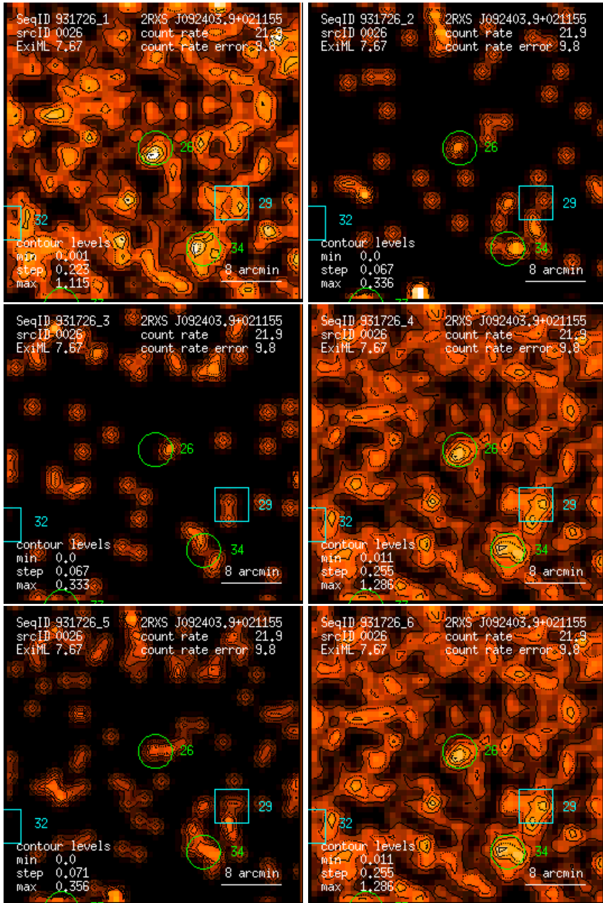
Figure 26: RASS 931726: detection 0026: band rate images, Gaussian filter: (1) PSPC channels 11 – 41, (2) 52 – 90, (3) 91 – 201, (4) 11 – 235, (5) 52 – 201, (6) 11 – 201. Broad band rates in counts/ks. Band rate contour levels in counts/ks/arcmin 2 .
