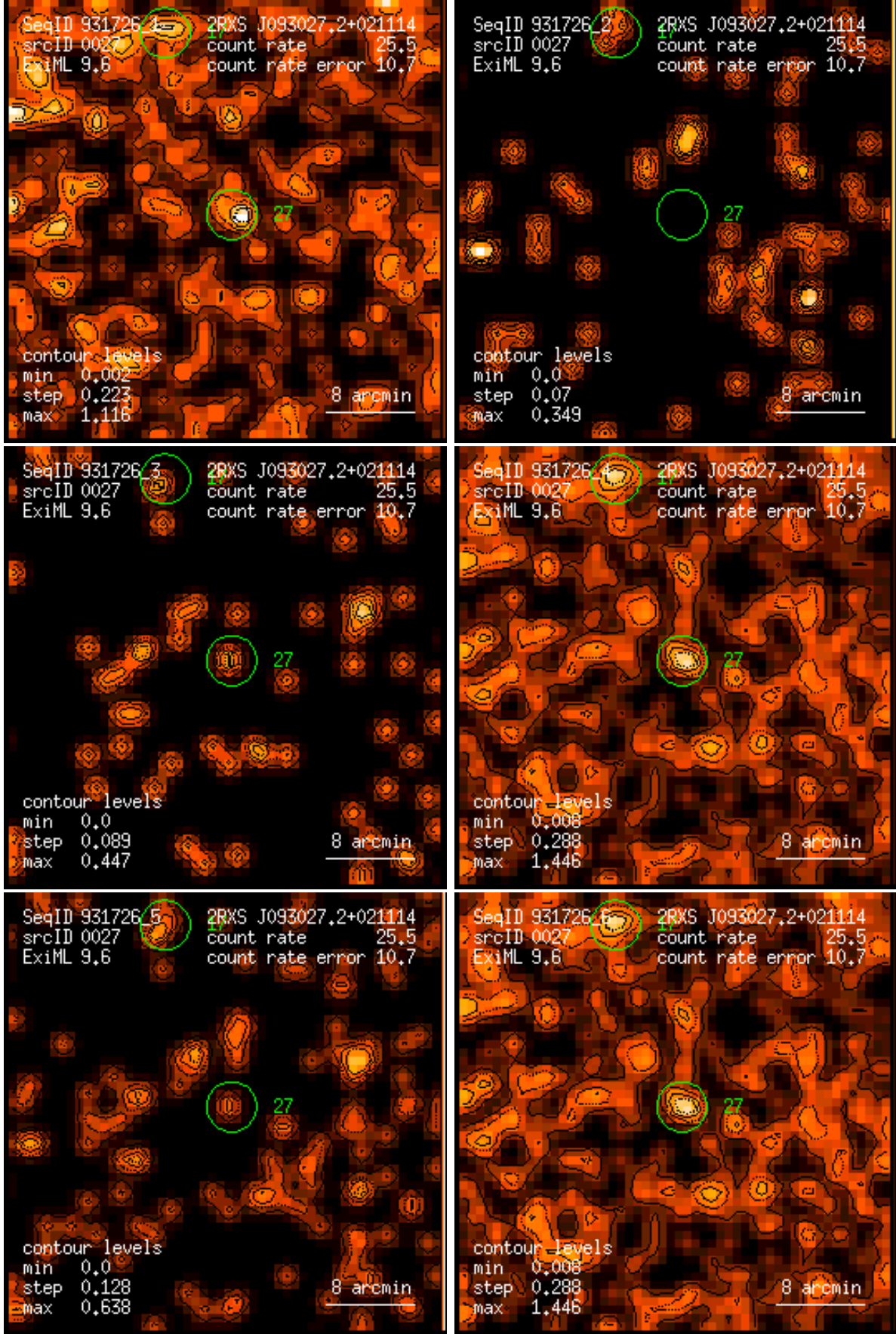
Figure 27: RASS 931726: detection 0027: band rate images, Gaussian filter: (1) PSPC channels 11 – 41, (2) 52 – 90, (3) 91 – 201, (4) 11 – 235, (5) 52 – 201, (6) 11 – 201. Broad band rates in counts/ks. Band rate contour levels in counts/ks/arcmin 2 .
