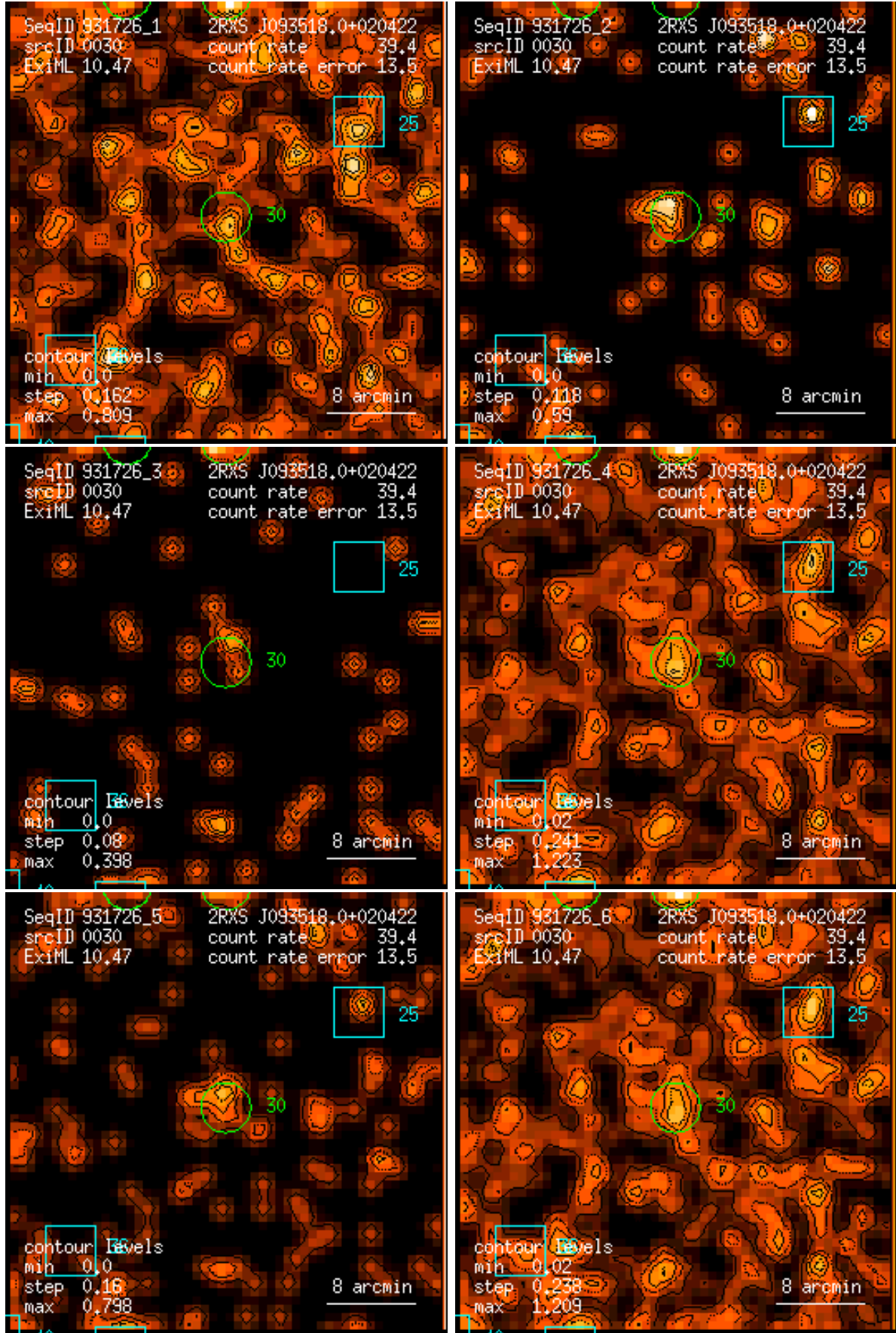
Figure 30: RASS 931726: detection 0030: band rate images, Gaussian filter: (1) PSPC channels 11 – 41, (2) 52 – 90, (3) 91 – 201, (4) 11 – 235, (5) 52 – 201, (6) 11 – 201. Broad band rates in counts/ks. Band rate contour levels in counts/ks/arcmin 2 .
