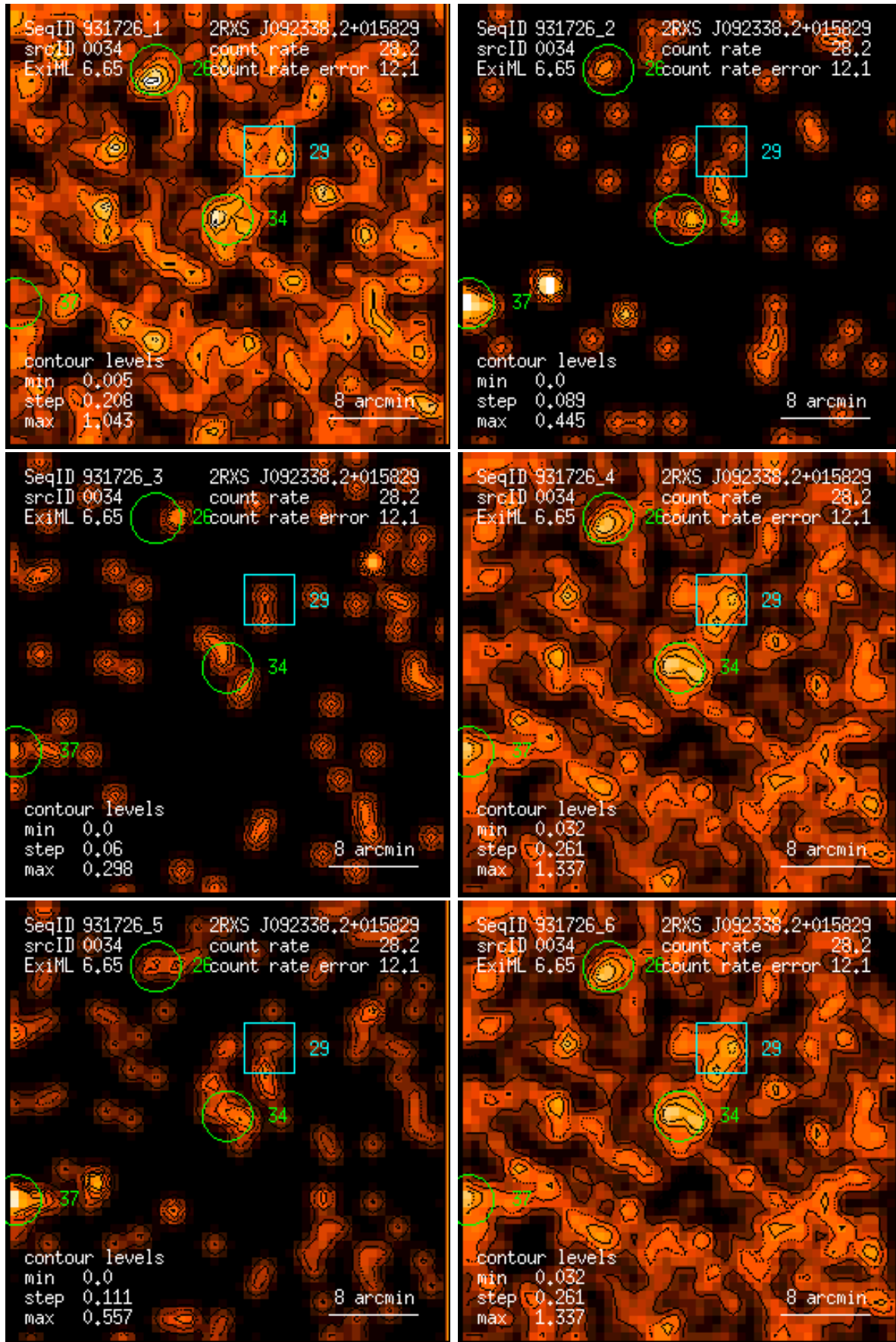
Figure 34: RASS 931726: detection 0034: band rate images, Gaussian filter: (1) PSPC channels 11 – 41, (2) 52 – 90, (3) 91 – 201, (4) 11 – 235, (5) 52 – 201, (6) 11 – 201. Broad band rates in counts/ks. Band rate contour levels in counts/ks/arcmin 2 .
