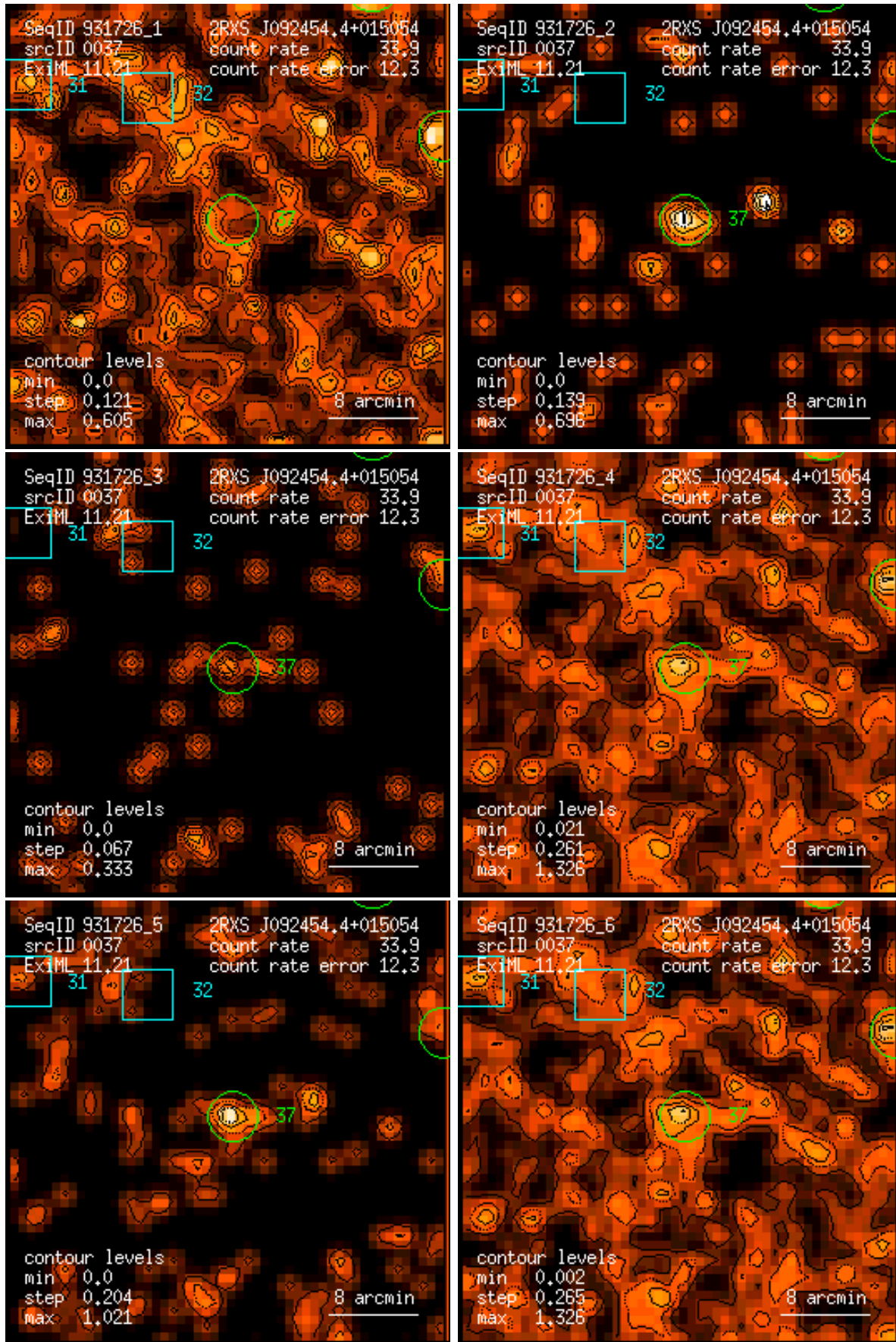
Figure 37: RASS 931726: detection 0037: band rate images, Gaussian filter: (1) PSPC channels 11 – 41, (2) 52 – 90, (3) 91 – 201, (4) 11 – 235, (5) 52 – 201, (6) 11 – 201. Broad band rates in counts/ks. Band rate contour levels in counts/ks/arcmin 2 .
