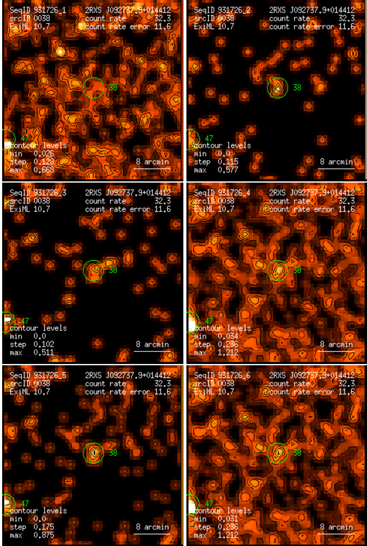
Figure 38: RASS 931726: detection 0038: band rate images, Gaussian filter: (1) PSPC channels 11 – 41, (2) 52 – 90, (3) 91 – 201, (4) 11 – 235, (5) 52 – 201, (6) 11 – 201. Broad band rates in counts/ks. Band rate contour levels in counts/ks/arcmin 2 .
