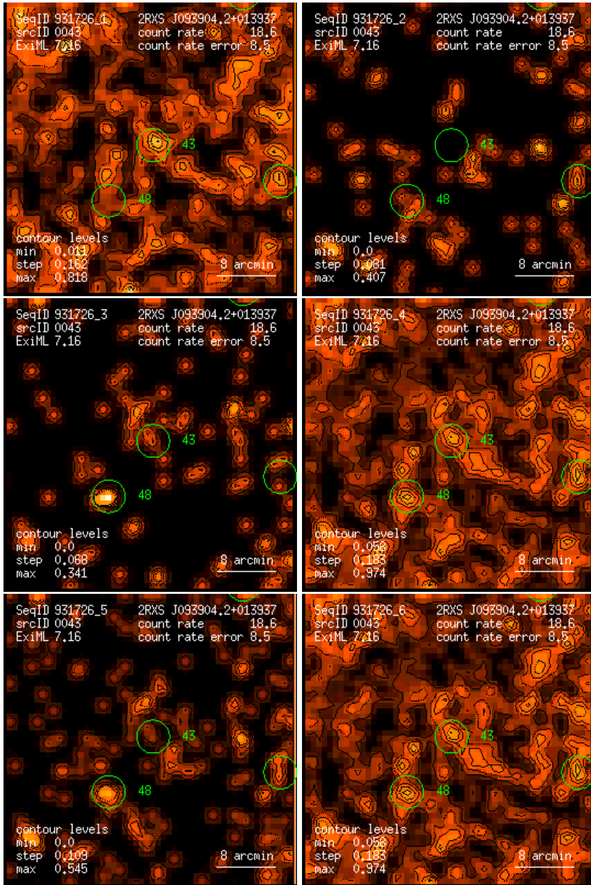
Figure 43: RASS 931726: detection 0043: band rate images, Gaussian filter: (1) PSPC channels 11 – 41, (2) 52 – 90, (3) 91 – 201, (4) 11 – 235, (5) 52 – 201, (6) 11 – 201. Broad band rates in counts/ks. Band rate contour levels in counts/ks/arcmin 2 .
