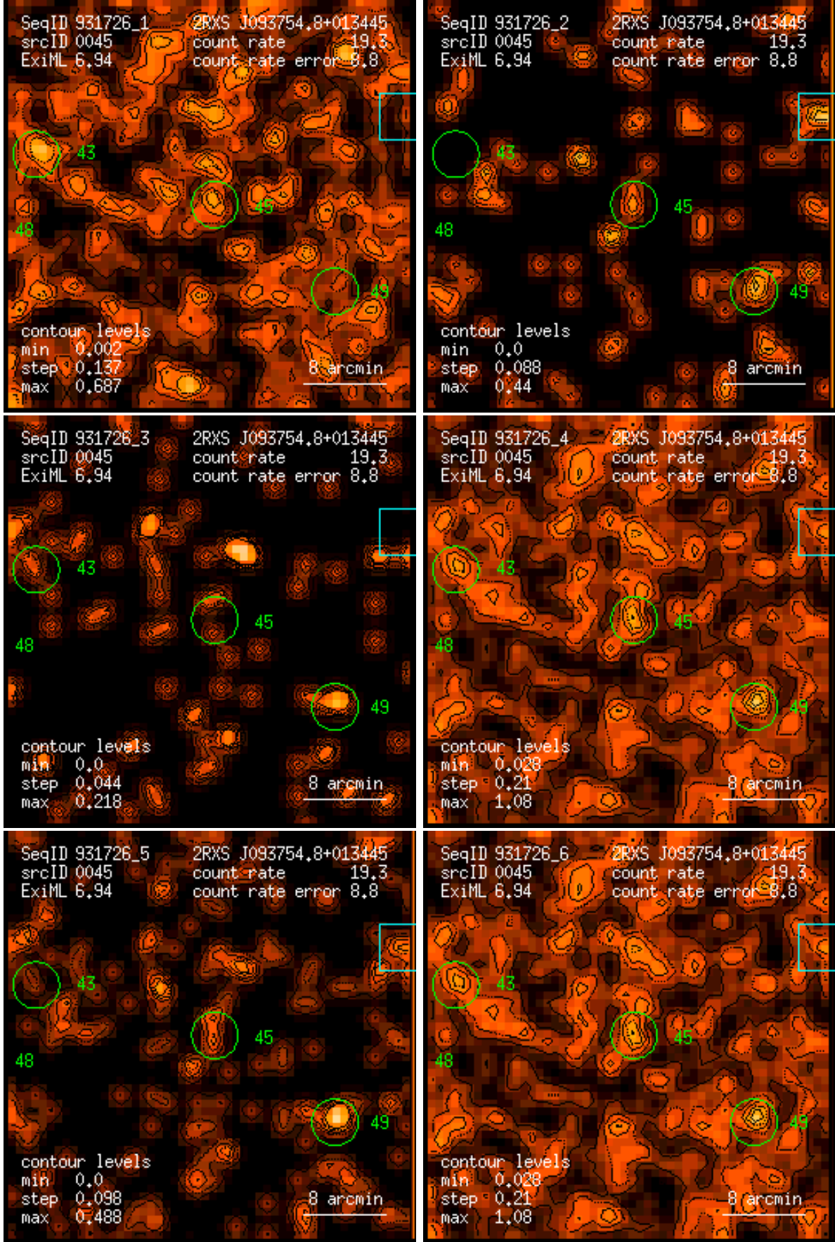
Figure 45: RASS 931726: detection 0045: band rate images, Gaussian filter: (1) PSPC channels 11 – 41, (2) 52 – 90, (3) 91 – 201, (4) 11 – 235, (5) 52 – 201, (6) 11 – 201. Broad band rates in counts/ks. Band rate contour levels in counts/ks/arcmin 2 .
