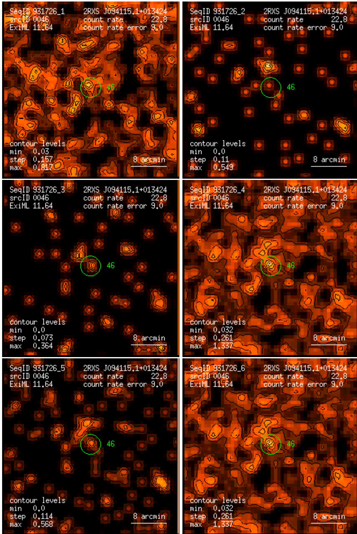
Figure 46: RASS 931726: detection 0046: band rate images, Gaussian filter: (1) PSPC channels 11 – 41, (2) 52 – 90, (3) 91 – 201, (4) 11 – 235, (5) 52 – 201, (6) 11 – 201. Broad band rates in counts/ks. Band rate contour levels in counts/ks/arcmin 2 .
