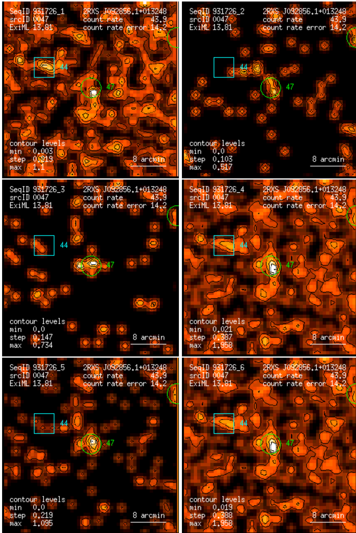
Figure 47: RASS 931726: detection 0047: band rate images, Gaussian filter: (1) PSPC channels 11 – 41, (2) 52 – 90, (3) 91 – 201, (4) 11 – 235, (5) 52 – 201, (6) 11 – 201. Broad band rates in counts/ks. Band rate contour levels in counts/ks/arcmin 2 .
