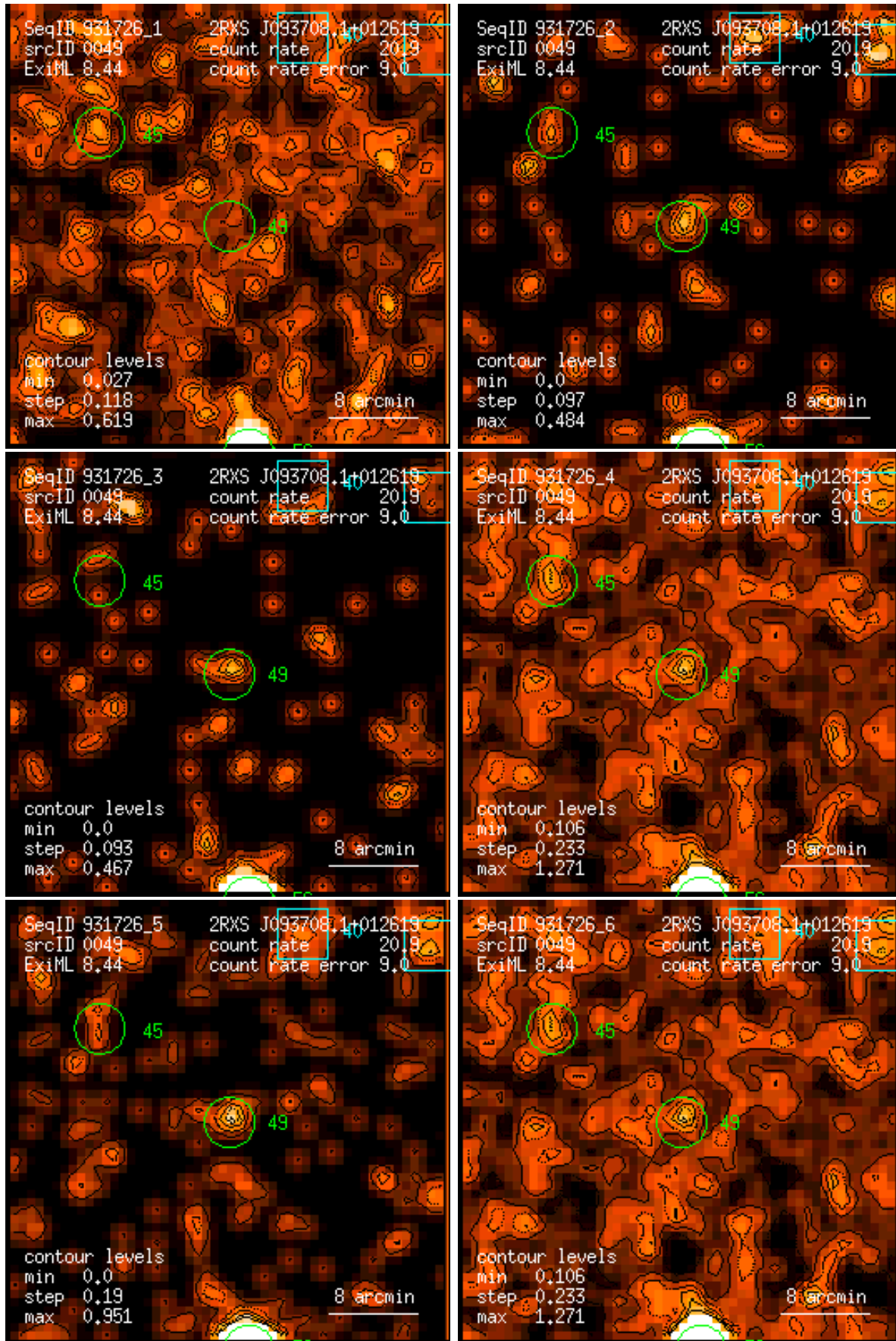
Figure 49: RASS 931726: detection 0049: band rate images, Gaussian filter: (1) PSPC channels 11 – 41, (2) 52 – 90, (3) 91 – 201, (4) 11 – 235, (5) 52 – 201, (6) 11 – 201. Broad band rates in counts/ks. Band rate contour levels in counts/ks/arcmin 2 .
