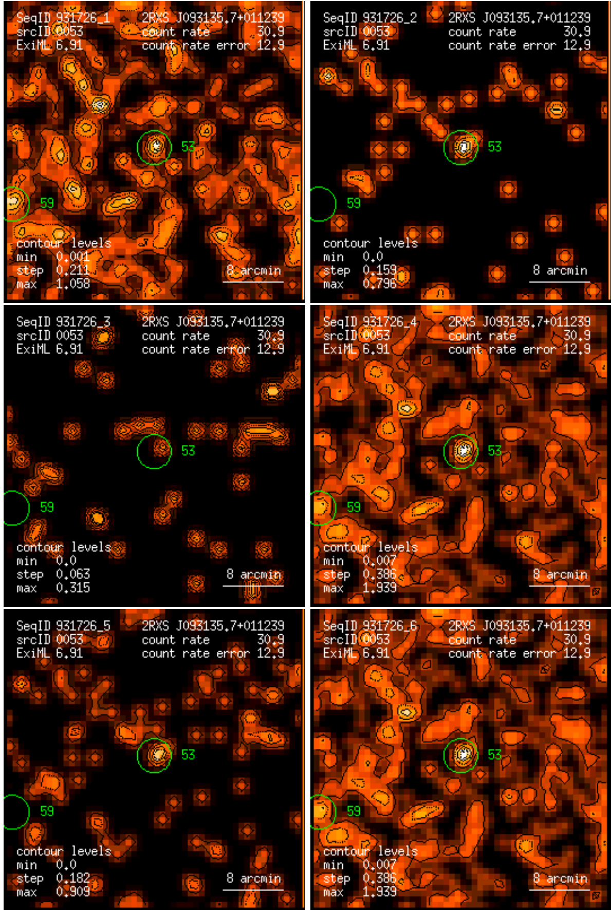
Figure 53: RASS 931726: detection 0053: band rate images, Gaussian filter: (1) PSPC channels 11 – 41, (2) 52 – 90, (3) 91 – 201, (4) 11 – 235, (5) 52 – 201, (6) 11 – 201. Broad band rates in counts/ks. Band rate contour levels in counts/ks/arcmin 2 .
